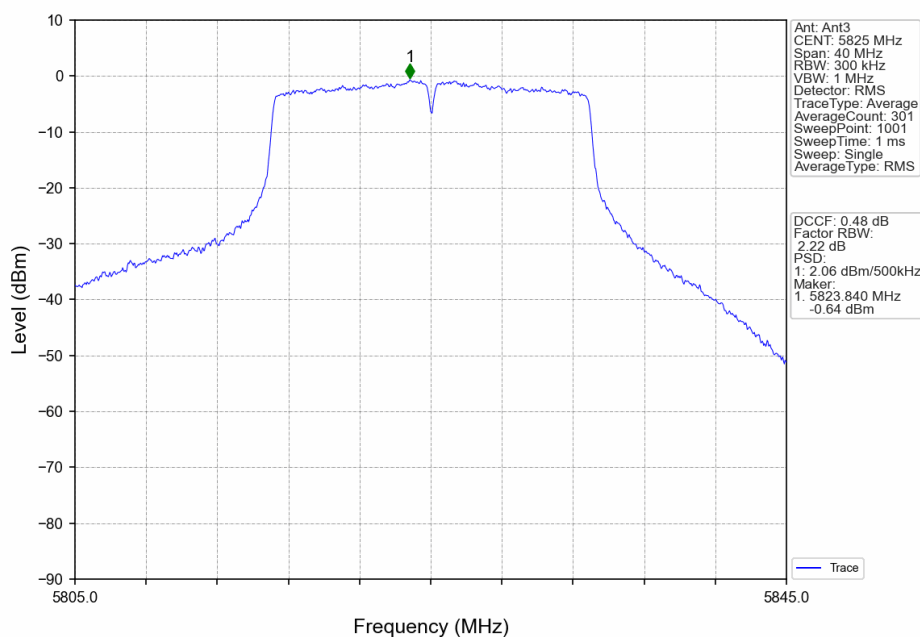
802.11ac(VHT20)_HCH_5825MHz_Ant3_NTNV
