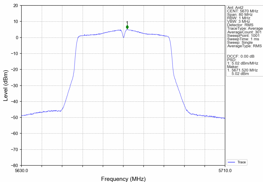
802.11n(HT40)_HCH_5670MHz_Ant2_NTNV
