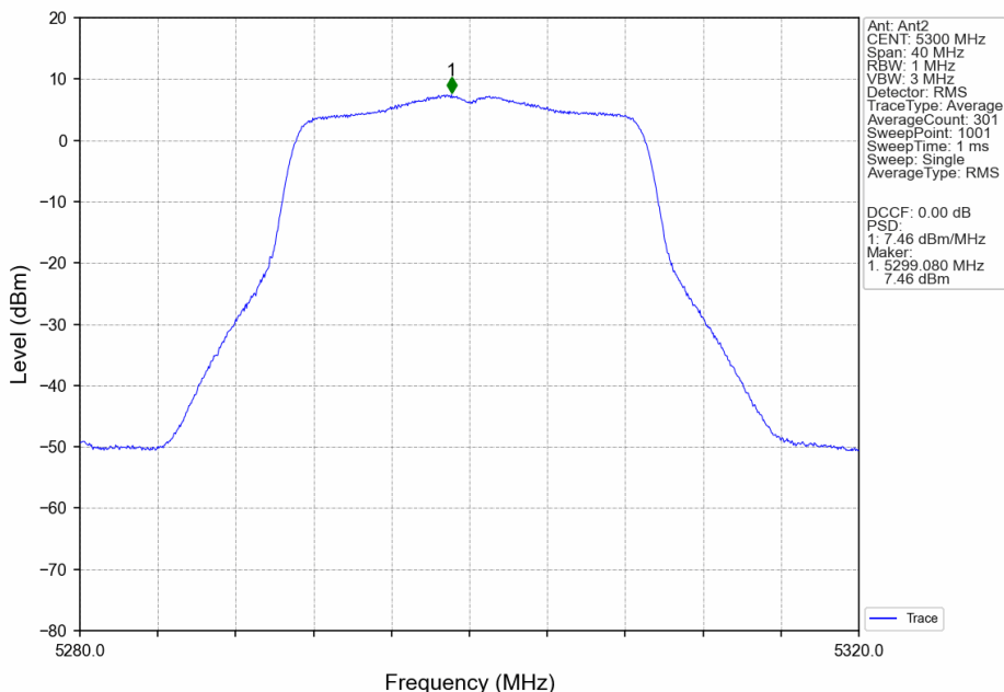
802.11ac(VHT20)_MCH_5300MHz_MIMO_NTNV
