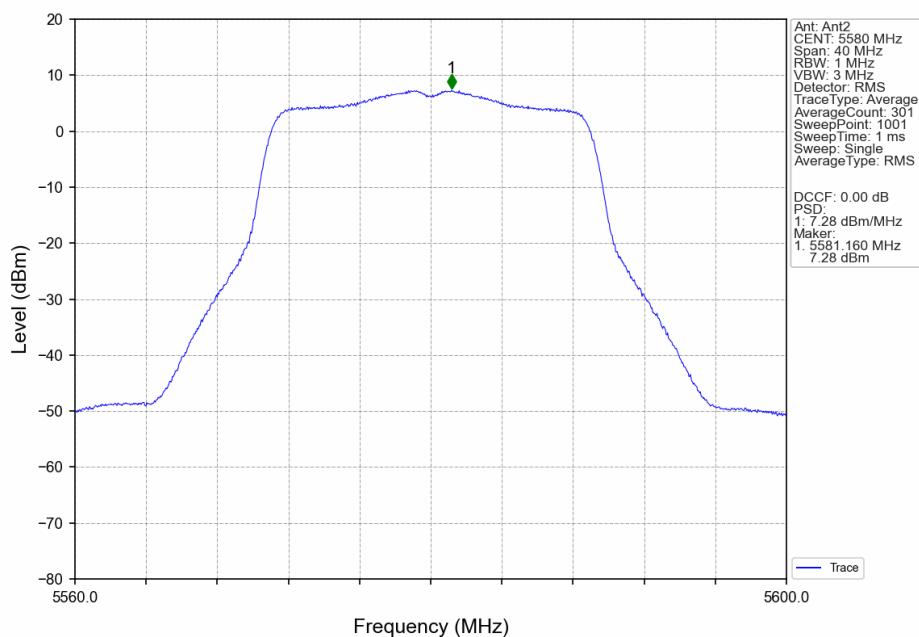
802.11ac(VHT20)_MCH_5580MHz_Ant2_NTNV
