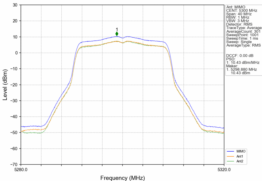
802.11ac(VHT20)_MCH_5300MHz_MIMO_NTNV
