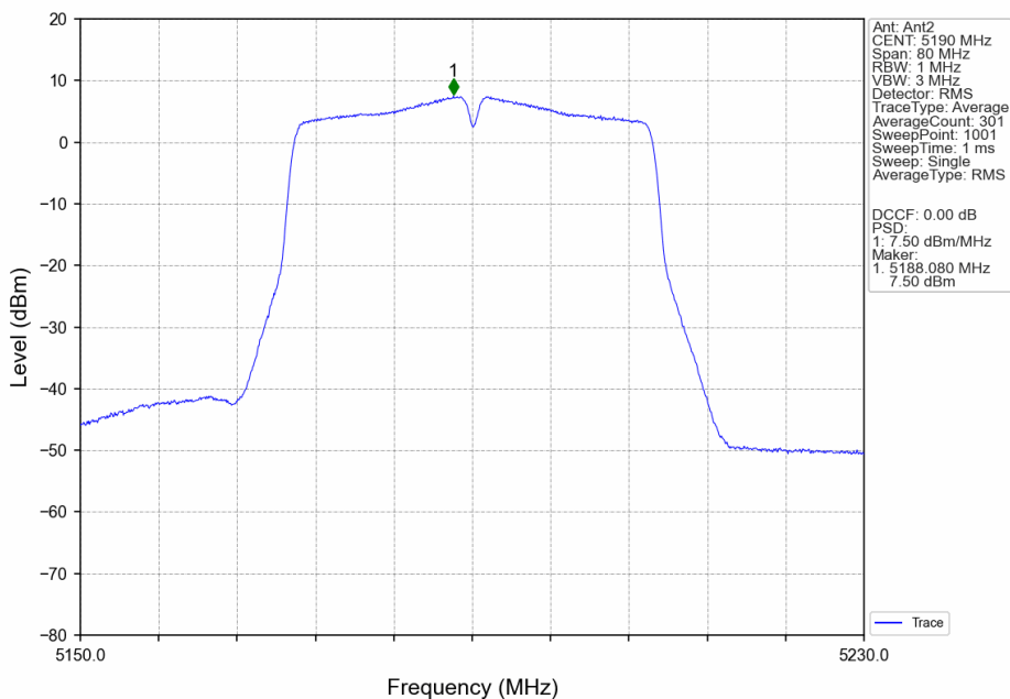
802.11ac(VHT40)_LCH_5190MHz_Ant2_NTNV
