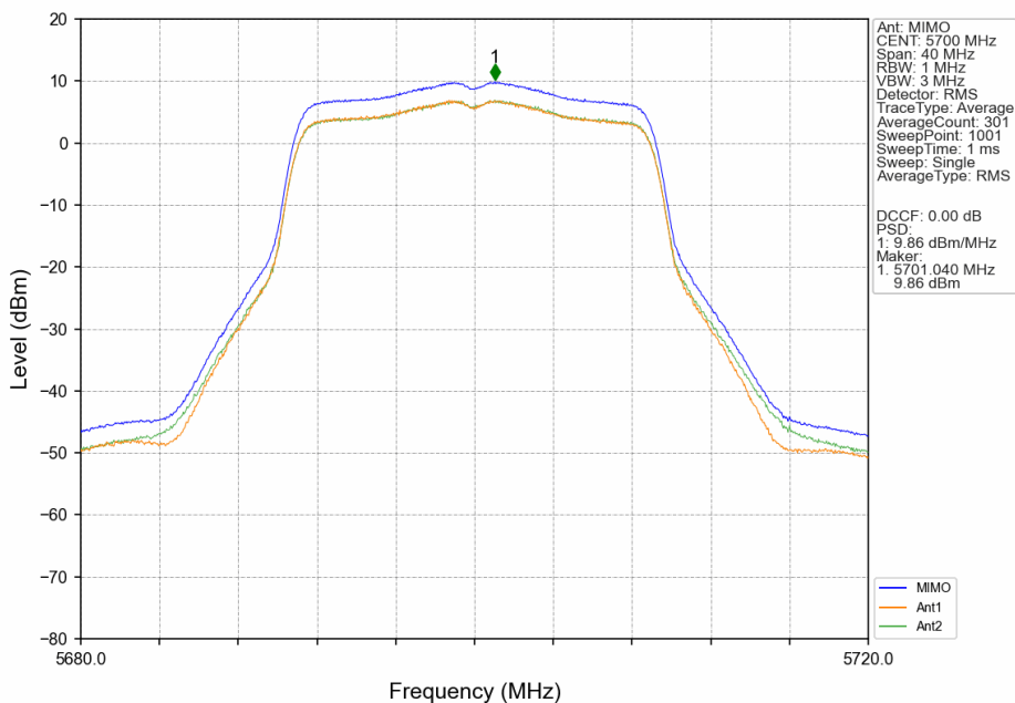
802.11ac(VHT20)_HCH_5700MHz_MIMO_NTNV
