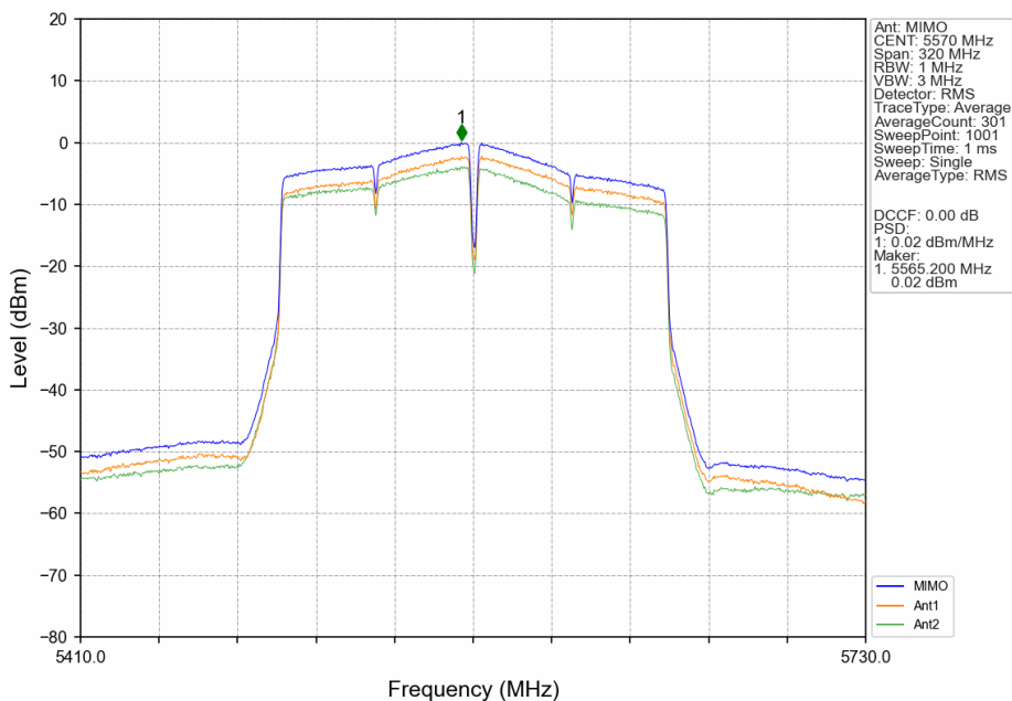
802.11ac(VHT160)_MCH_5570MHz_MIMO_NTNV
