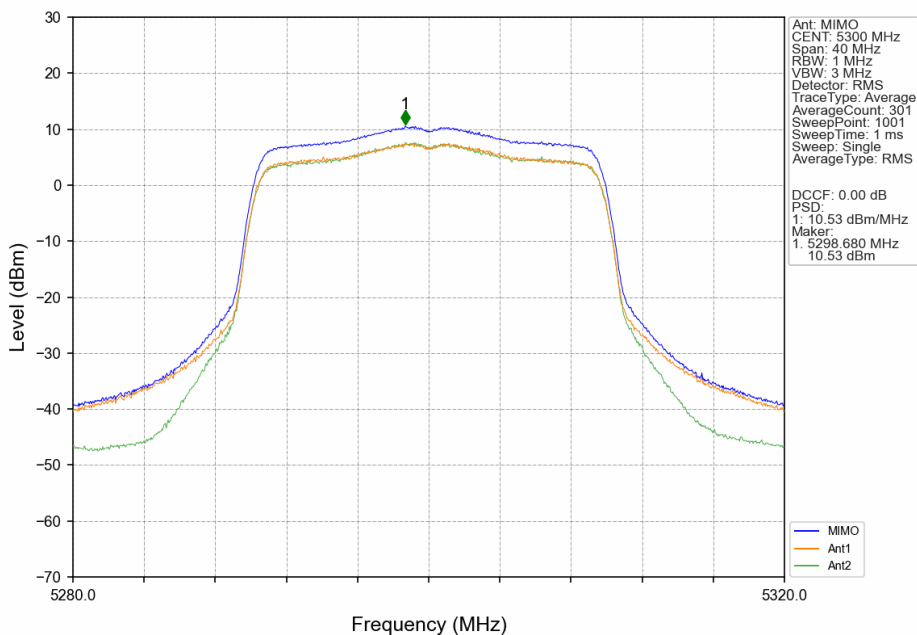
802.11ax(HEW20)_MCH_5300MHz_RU242_Left_MIMO_NTNV
