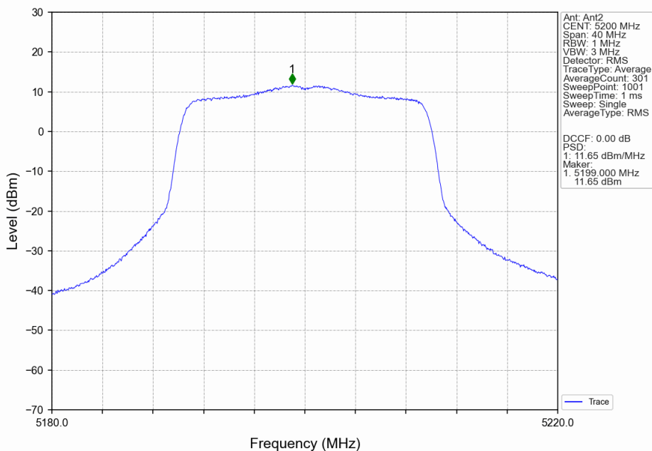
802.11ax(HEW20)_MCH_5200MHz_RU242_Left_Ant2_NTNV
