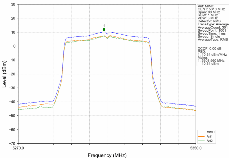
802.11ax(HEW40)_HCH_5310MHz_RU484_Left_MIMO_NTNV
