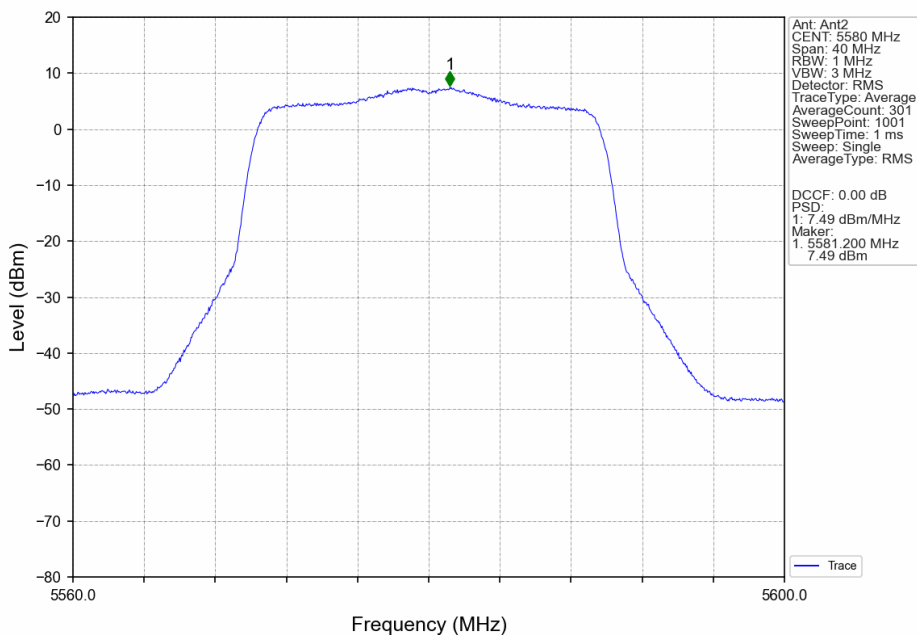
802.11ax(HEW20)_MCH_5580MHz_RU242_Left_Ant2_NTNV
