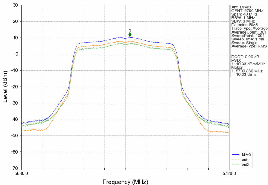
802.11ax(HEW20)_HCH_5700MHz_RU242_Left_MIMO_NTNV
