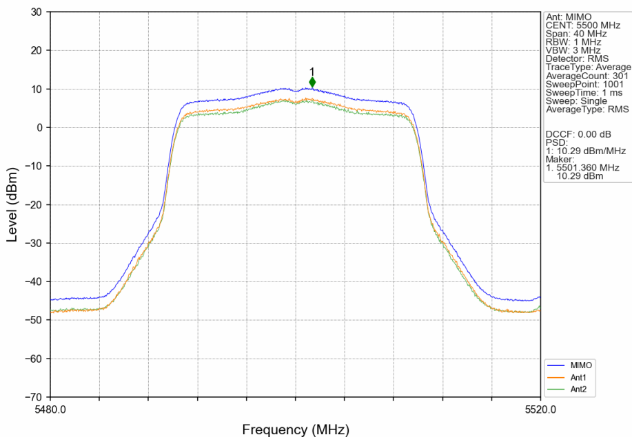
802.11ax(HEW20)_LCH_5500MHz_RU242_Left_MIMO_NTNV
