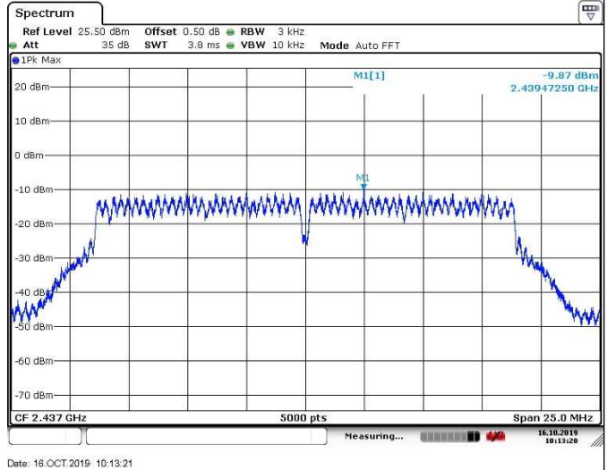
Channel 06 (2437MHz)
