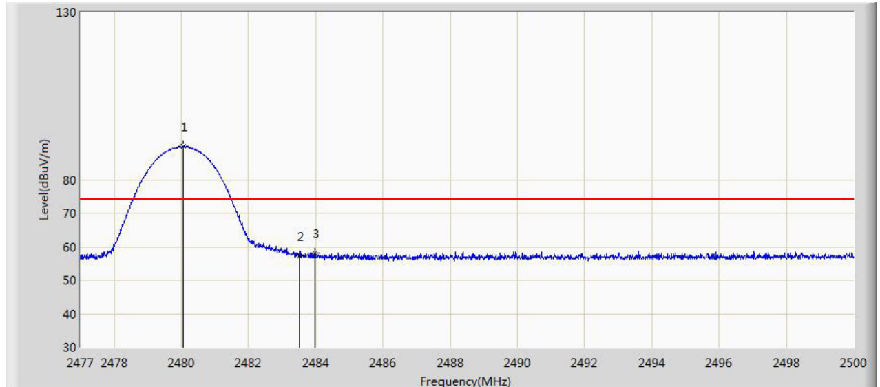
Figure 47: Band Edge, 3-DH5, 2480MHz, Vertical, PK
