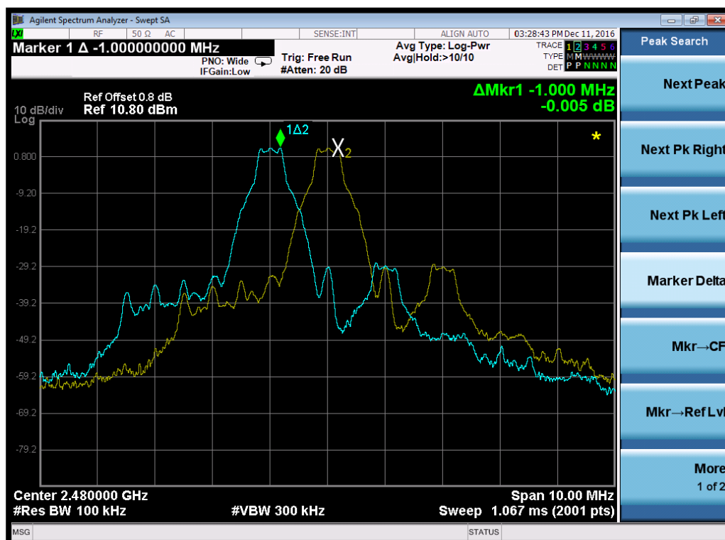
Figure 51: Frequency Separation, DH5, 2480MHz
