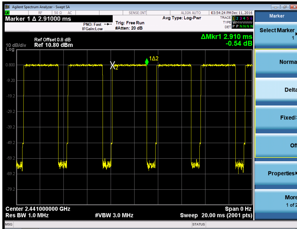
Figure 63: Time of Occupancy, 3-DH5, 2441MHz
