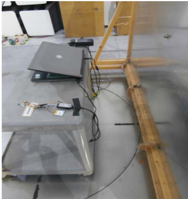
AC Line Conducted Emissions
