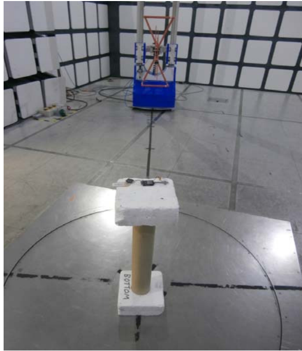
Radiated Emissions 30 MHz to 1 GHz
