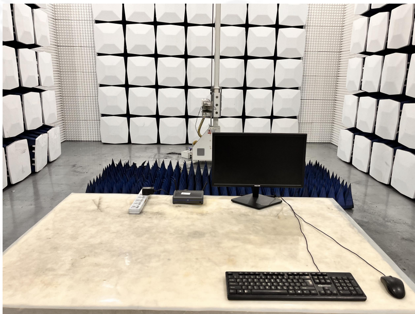
RE-above 1G
