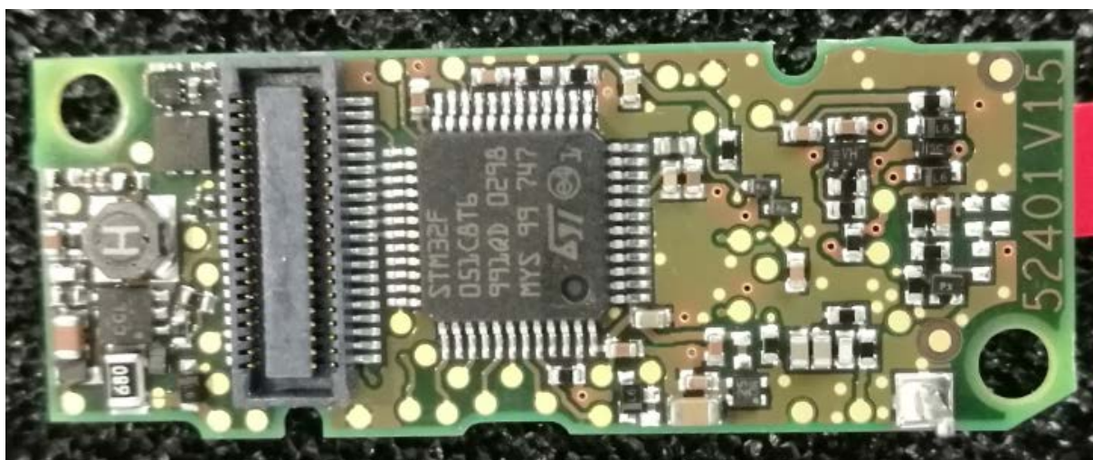
Bodenprint PCB, connector side
