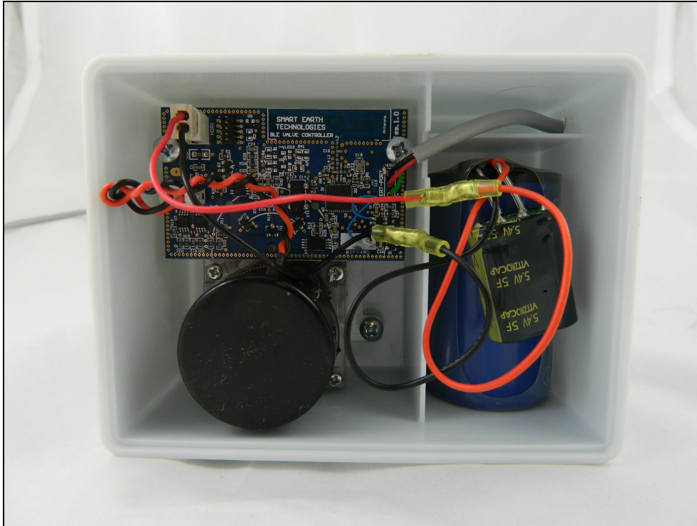
Figure 1: Internal Photo
