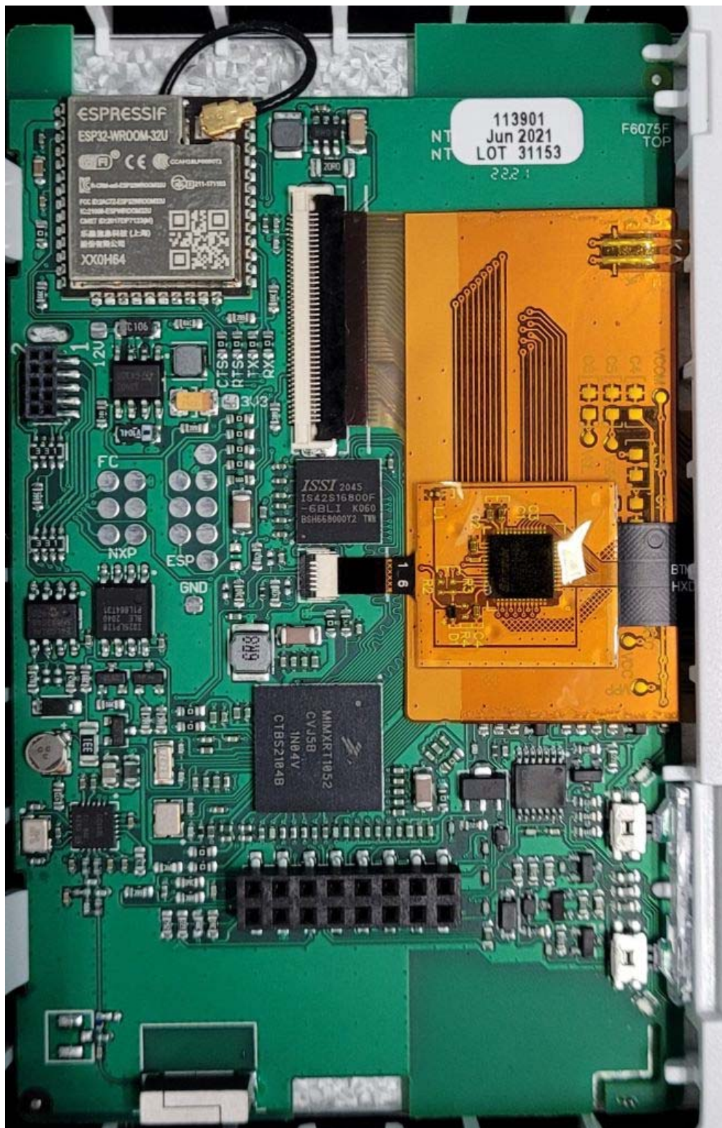
Figure E22.6 – F6075D – Top View
