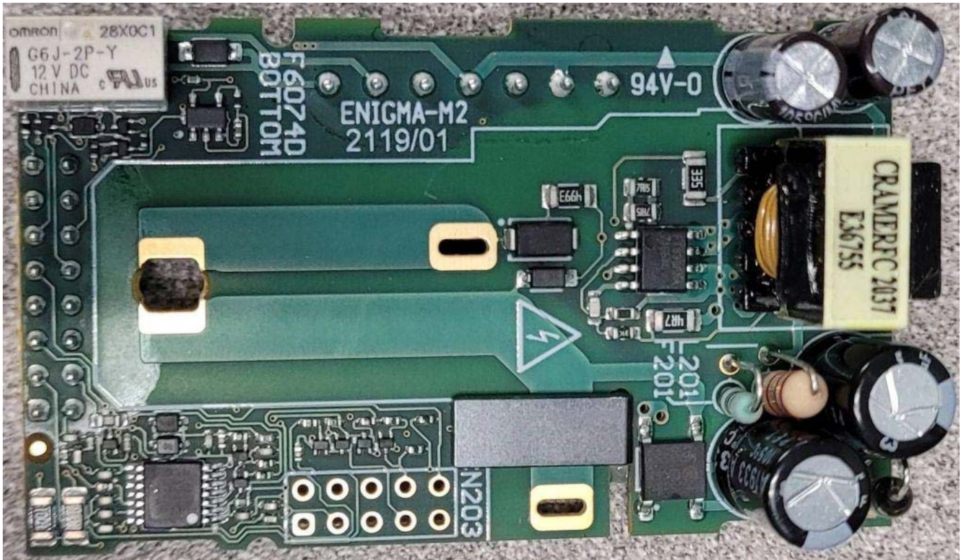
Figure E22.5 – F6074D – Bottom View
