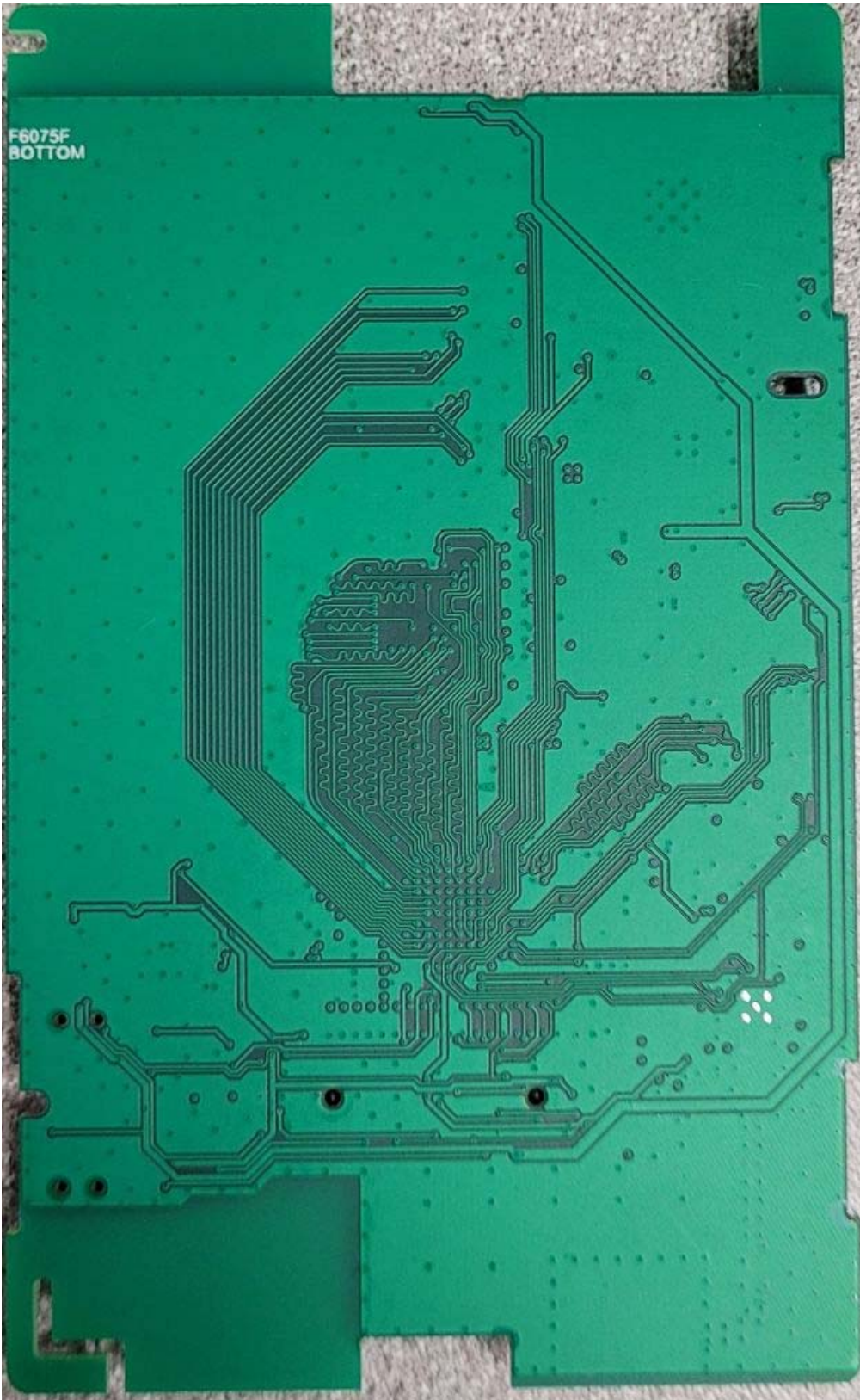
Figure E22.7 – F6075D – Bottom View
