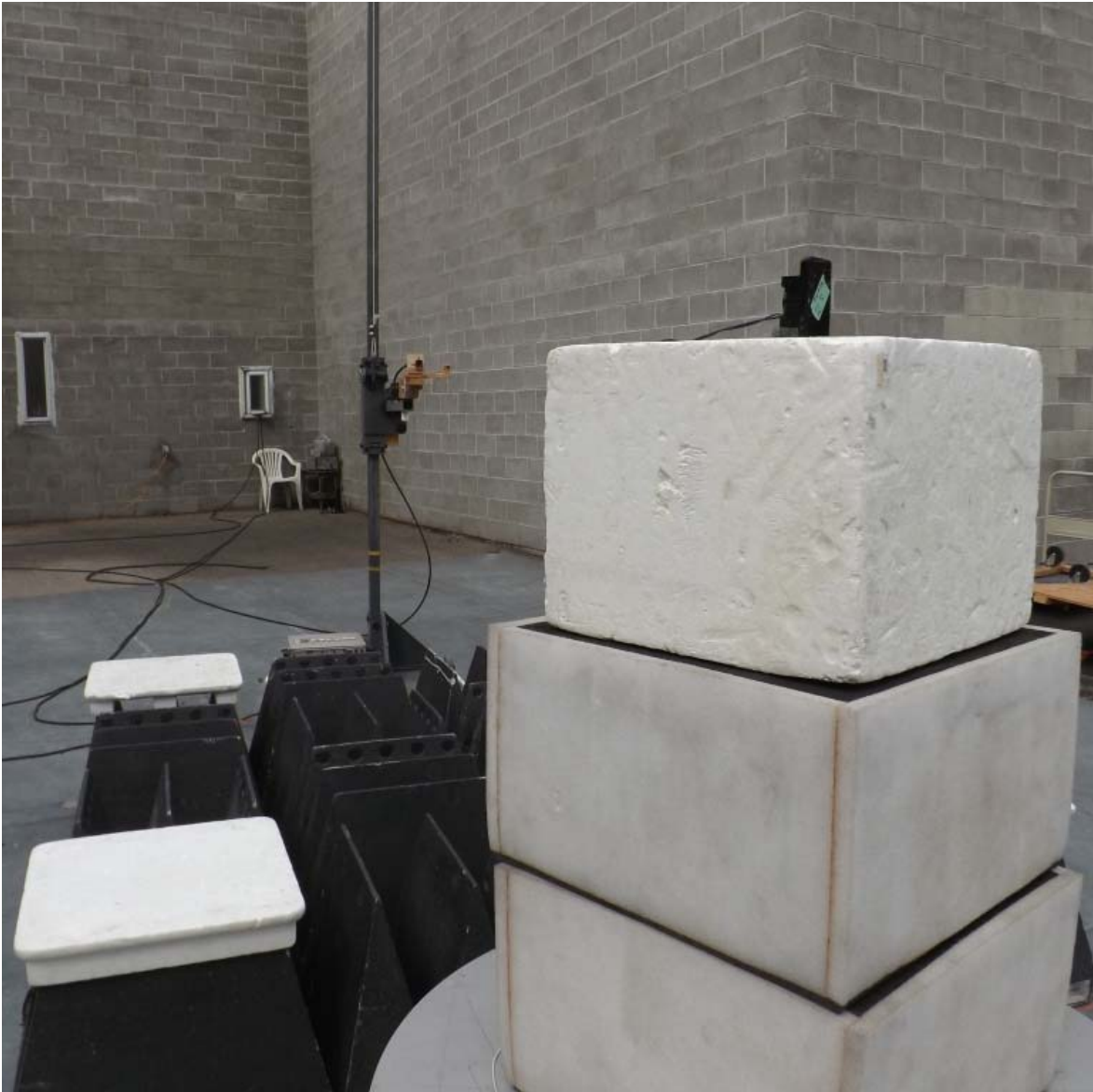
Figure E23.4 – Setup, Radiated Measurements Below 18 – 26GHz
