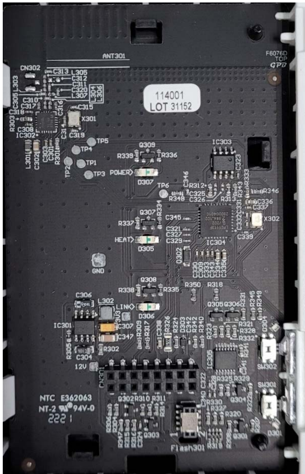
Figure E22.6 – F6076D – Top View
