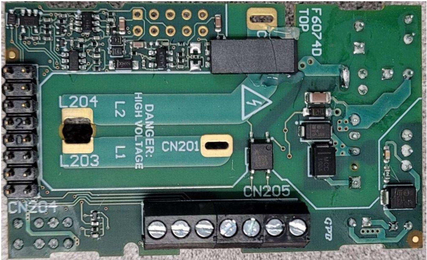
Figure E22.4 – F6074D – Top View
