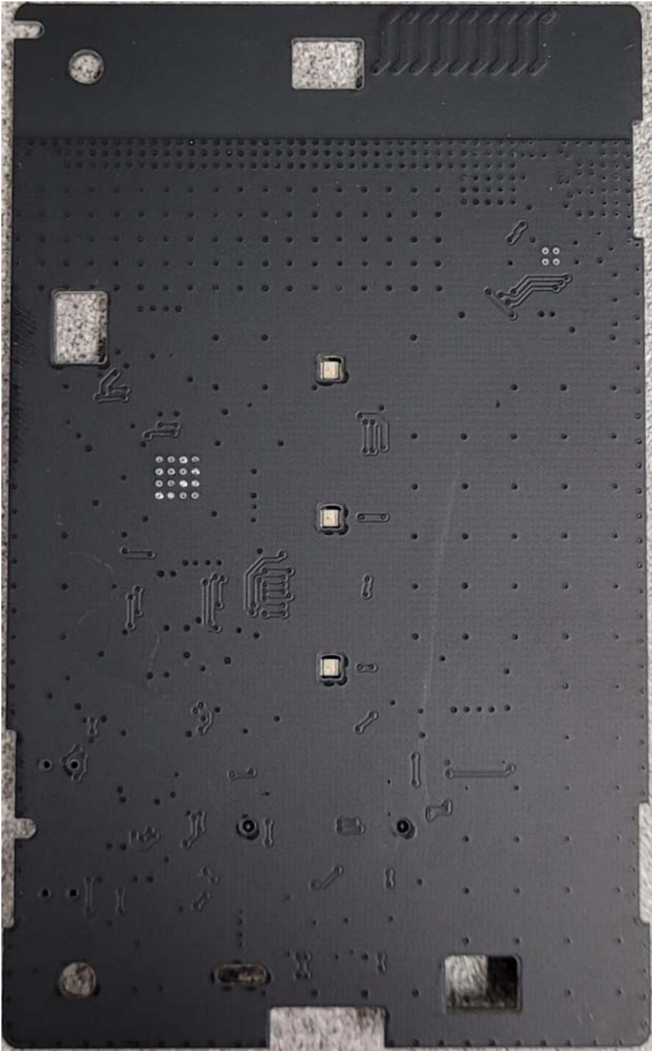
Figure E22.7 – F6076D – Bottom View
