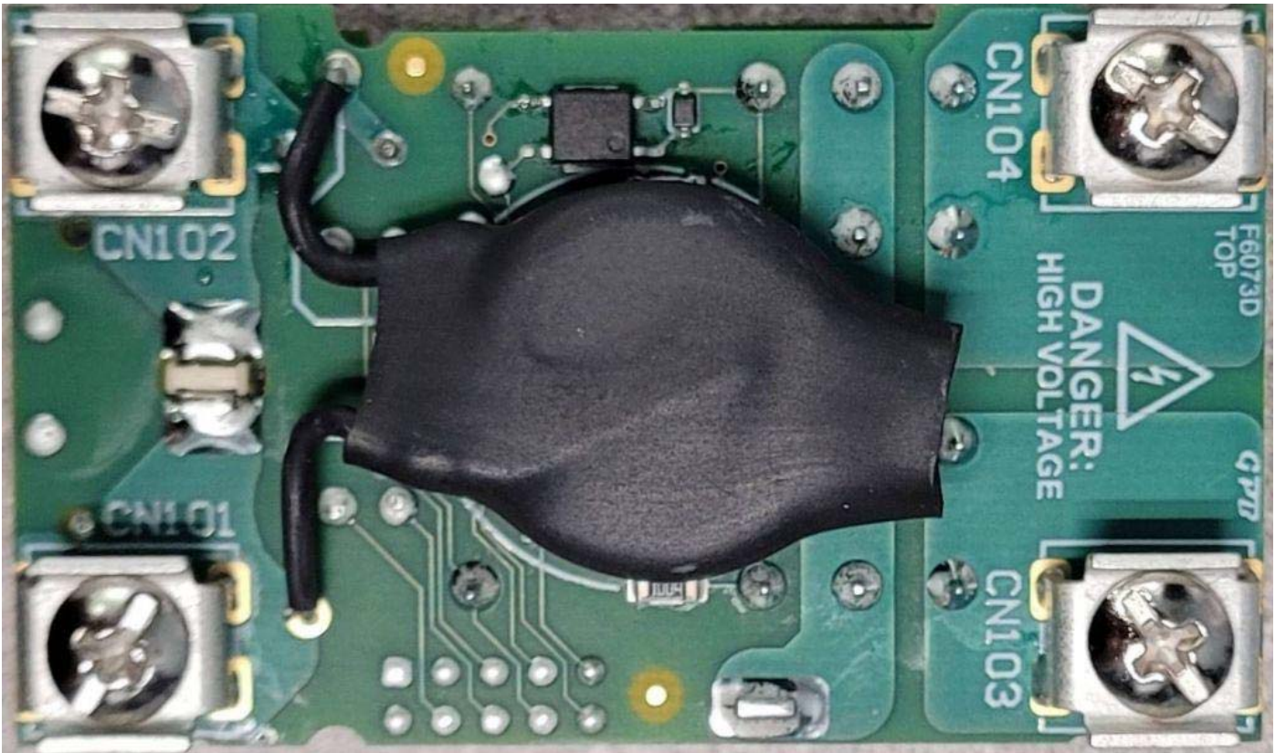
Figure E22.2 – F6073D – Bottom View
