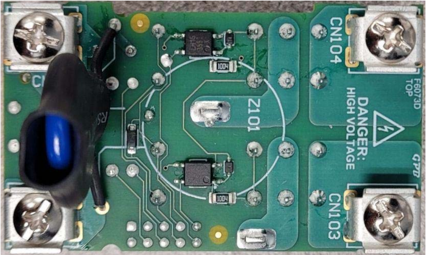
Figure E22.3 – F6073D – Bottom View – MOV Moved
