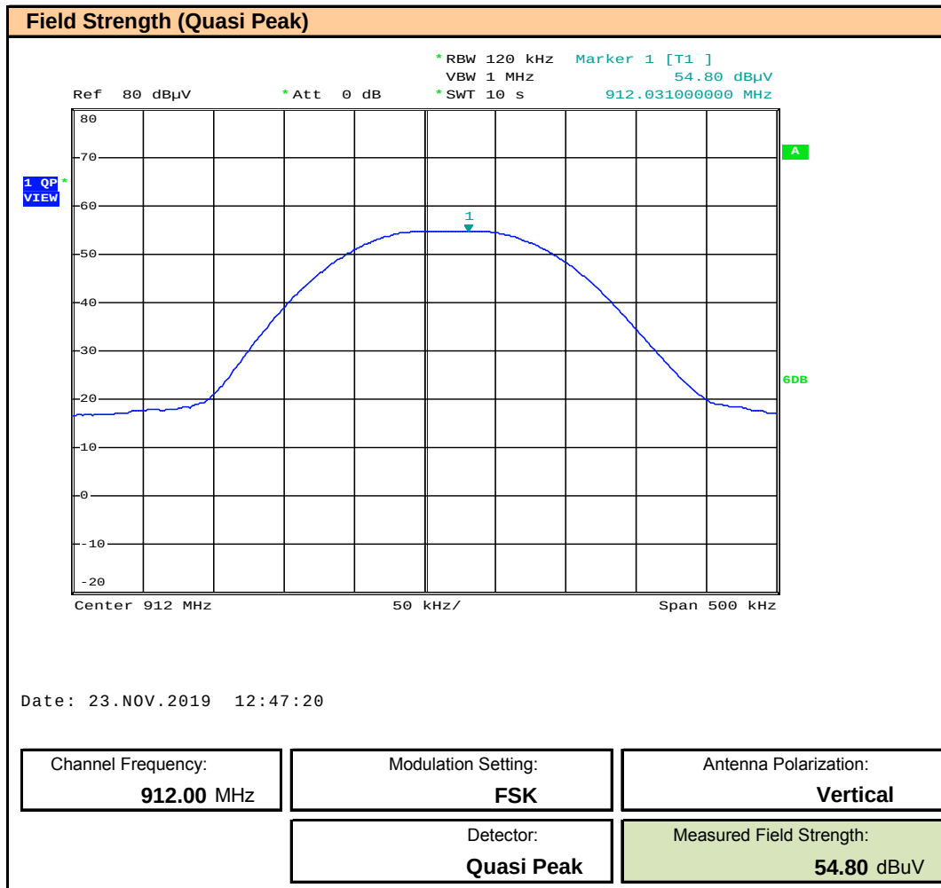
Plot 9.4 – Field Strength – Quasi Peak - Vertical
