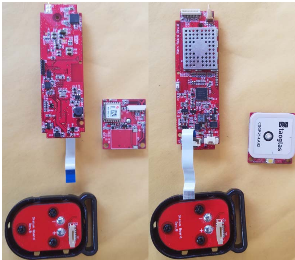
Figure 1 - Specifi-Kali Dog Tracking System – PWB's – Top & Bottom
