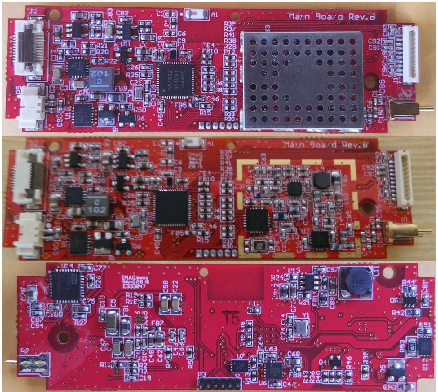
Figure 2 - Specifi-Kali Dog Tracking System - Main PWB – Top, Top w/o Shield, Bottom
