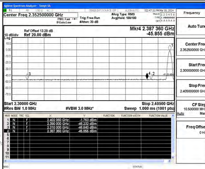
2DH5_Ant_Low_2402_Peak
