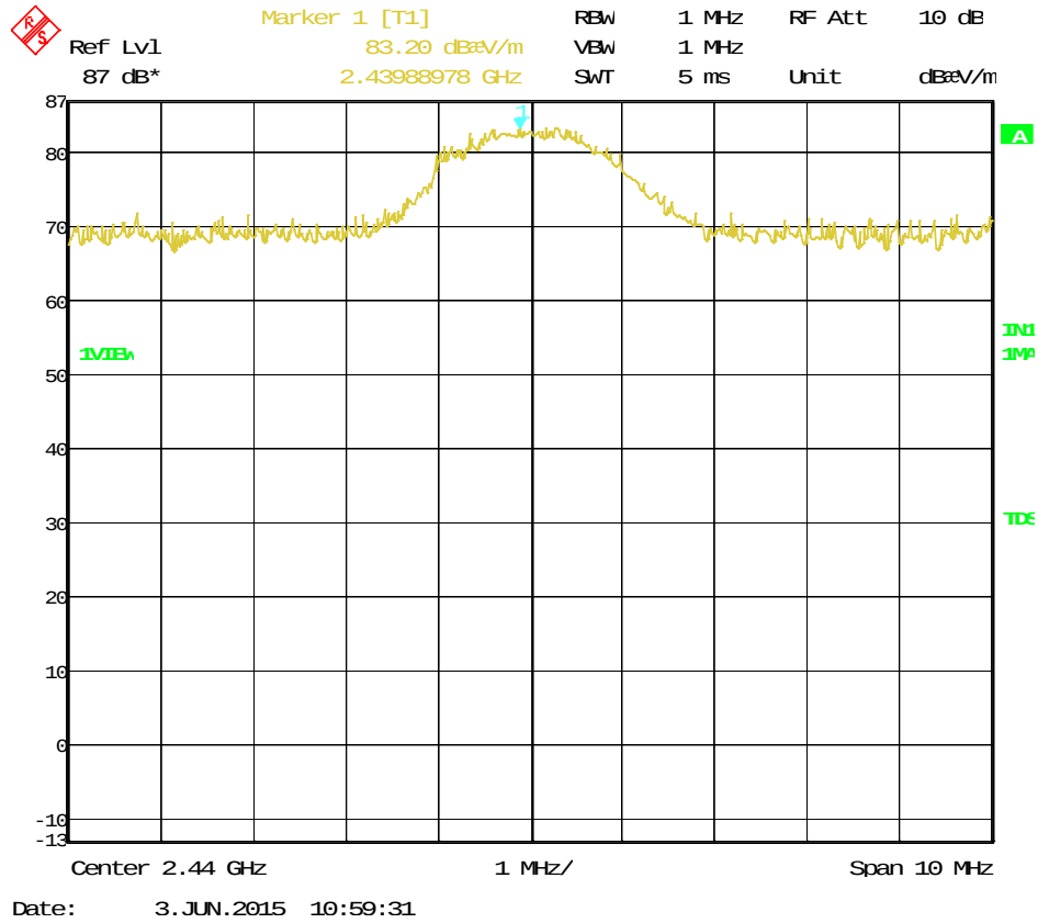
Figure 24 2440.0 MHz – Vertical
