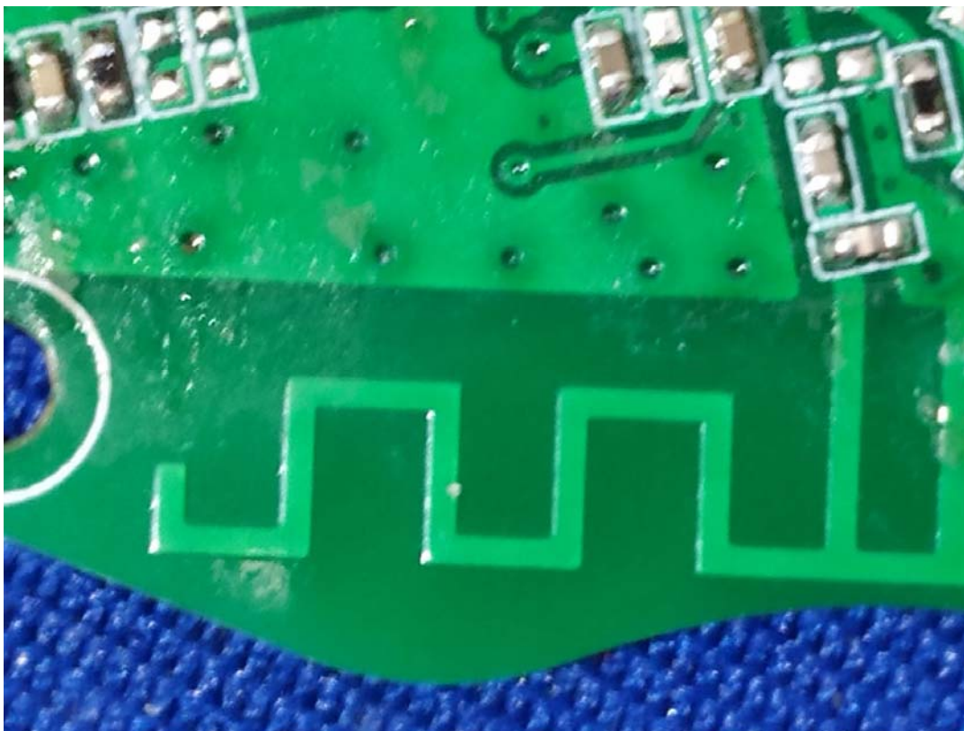
BT antenna
