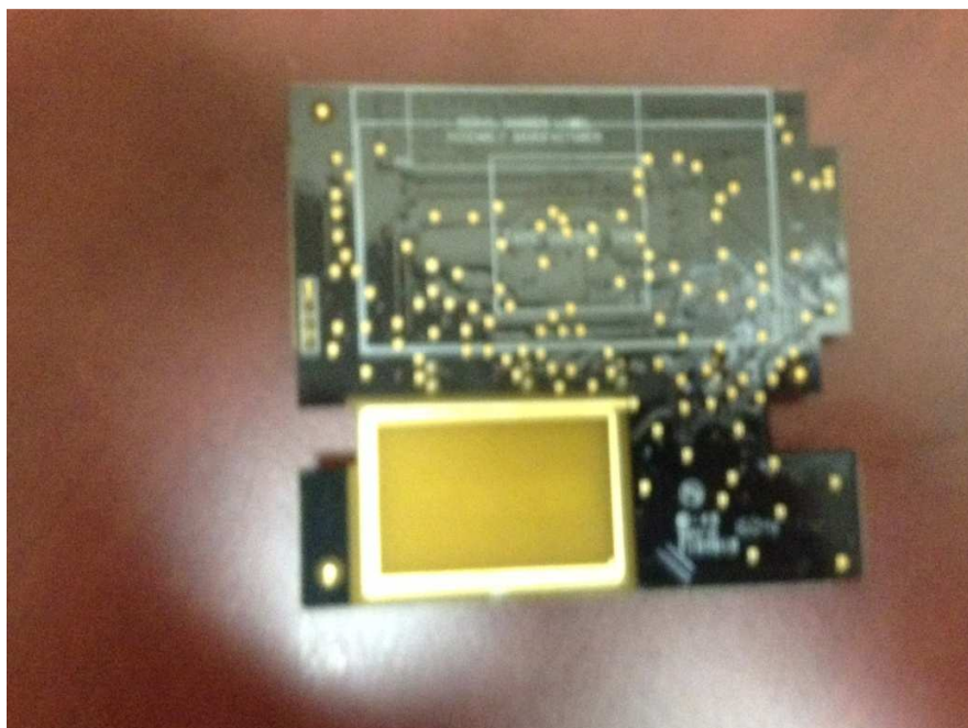
Top PCB of KP-8IN-1REL- solders side
