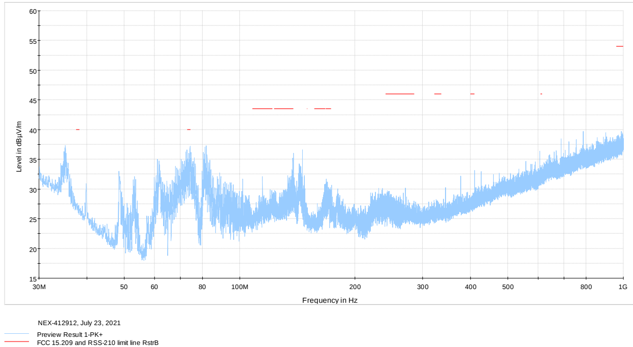
Figure 7.1-1: Radiated emissions spectral plot (30 to 1000 MHz)
