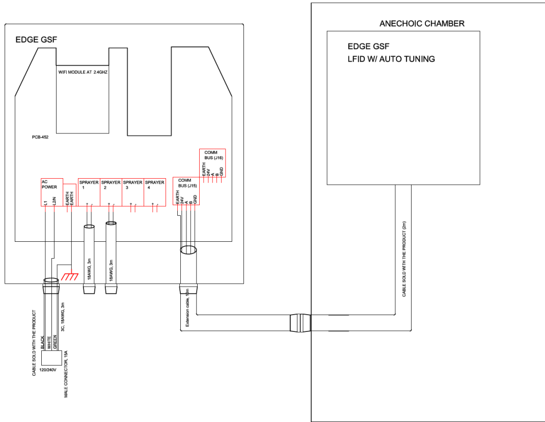
Figure 5.6-1: block diagram
