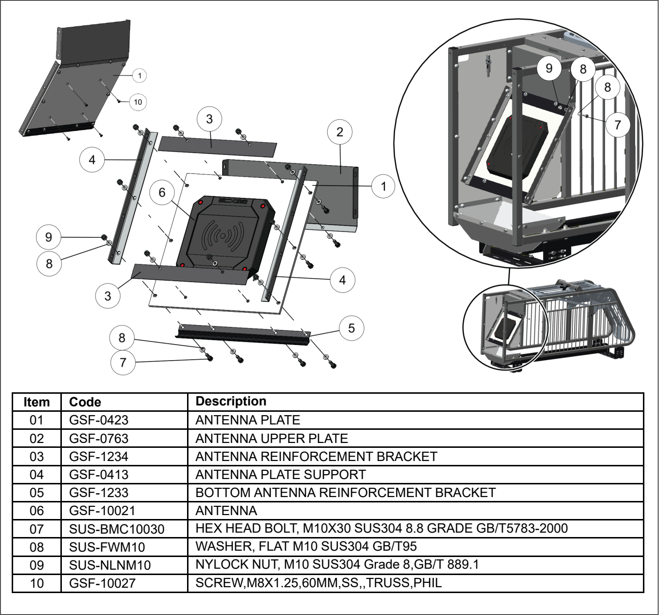
Figure 2-1 Mounting the antenna
