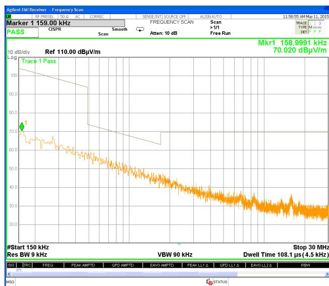
Plot # 4. Spurious emissions scan 0.15 MHz – 30 MHz.
