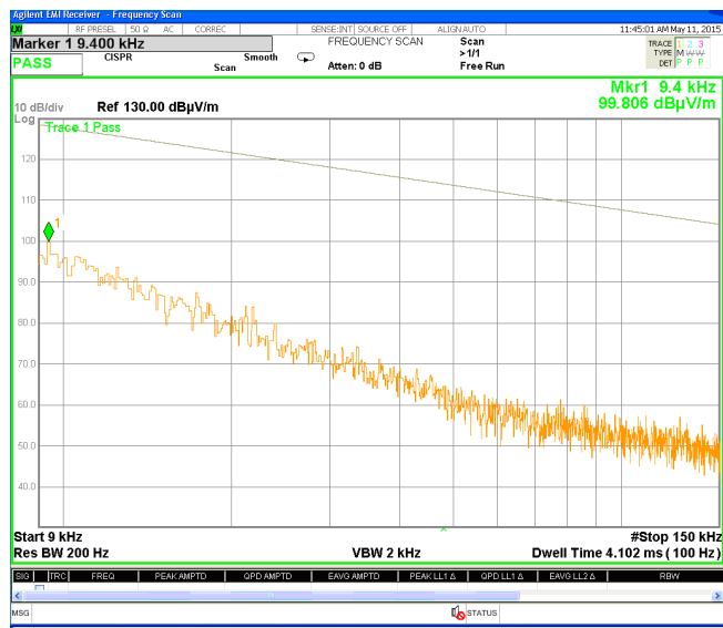
Plot # 3. Spurious emissions scan 0.009 MHz – 0.15 MHz.
