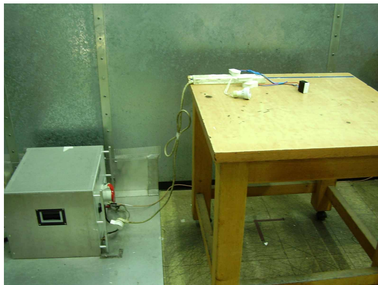
Photo 4. Conducted emission test setup
