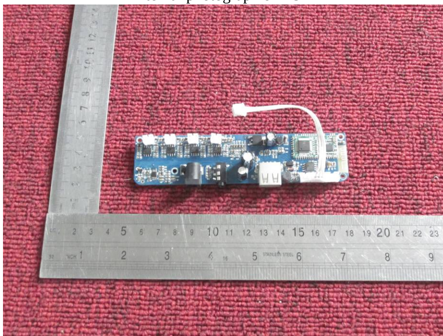
nternal photograph of EUT
