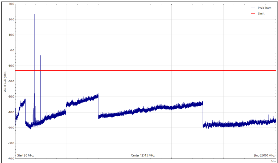
Figure 2 - BLE 2440 MHz & CAT M1 LTE B2, 30 MHz to 25 GHz, Horizontal (Peak)
