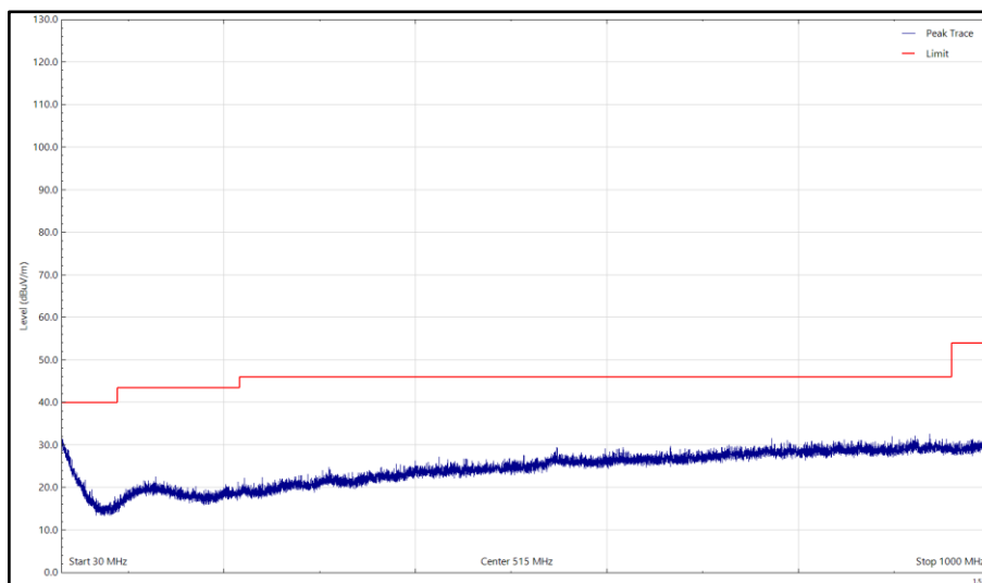
Figure 16 - 2440 MHz (CH17), LE1M, 30 MHz to 1 GHz, Horizontal (Peak)
