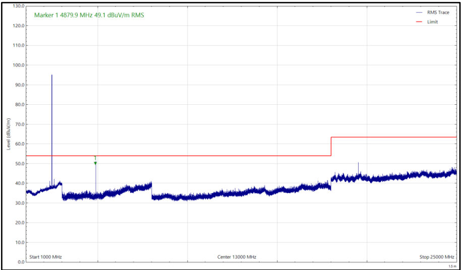
Figure 18 - 2440 MHz (CH17), LE1M, 1 GHz to 25 GHz, Horizontal (rms)
