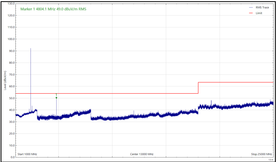
Figure 12 - 2402 MHz (CH37), LE1M, 1 GHz to 25 GHz, Horizontal (rms)
