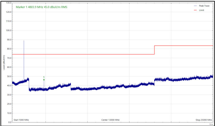
Figure 14 - 2402 MHz (CH37), LE1M, 1 GHz to 25 GHz, Vertical (Peak)
