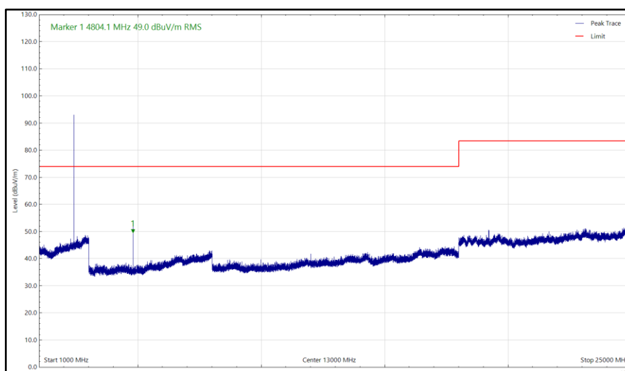
Figure 11 - 2402 MHz (CH37), LE1M, 1 GHz to 25 GHz, Horizontal (Peak)
