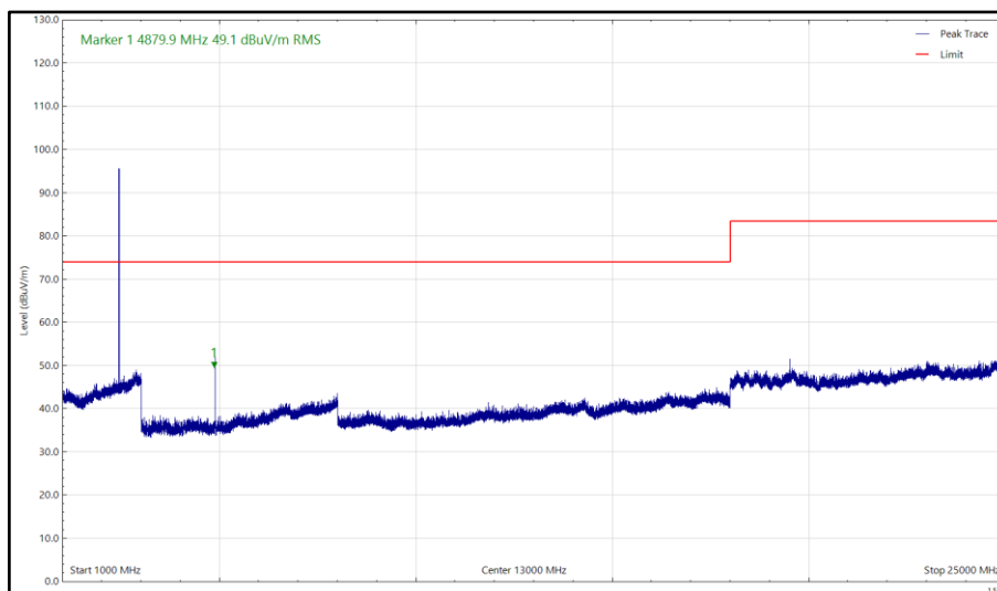
Figure 17 - 2440 MHz (CH17), LE1M, 1 GHz to 25 GHz, Horizontal (Peak)
