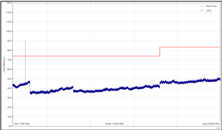
Figure 26 - 2480 MHz (CH39), LE1M, 1 GHz to 25 GHz, Vertical (Peak)
