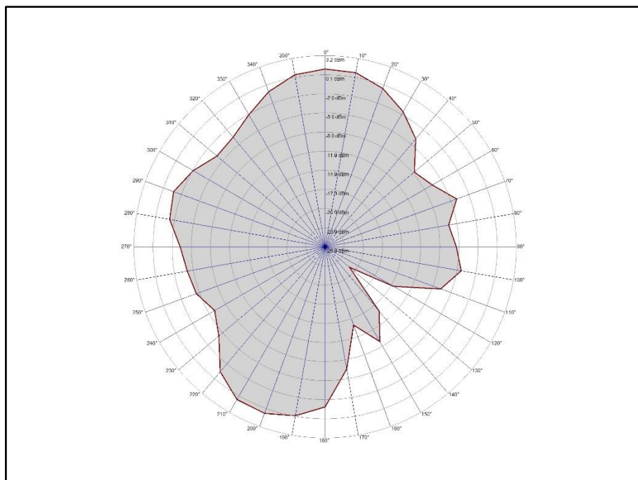
Figure 5 - 2440 MHz, Horizontal
