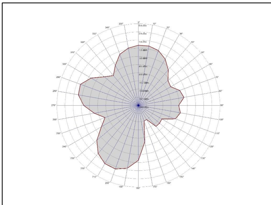
Figure 7 - 2480 MHz, Horizontal
