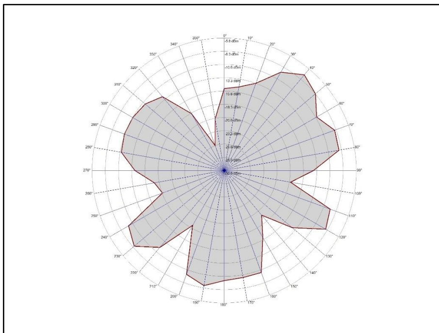
Figure 6 - 2440 MHz, Vertical
