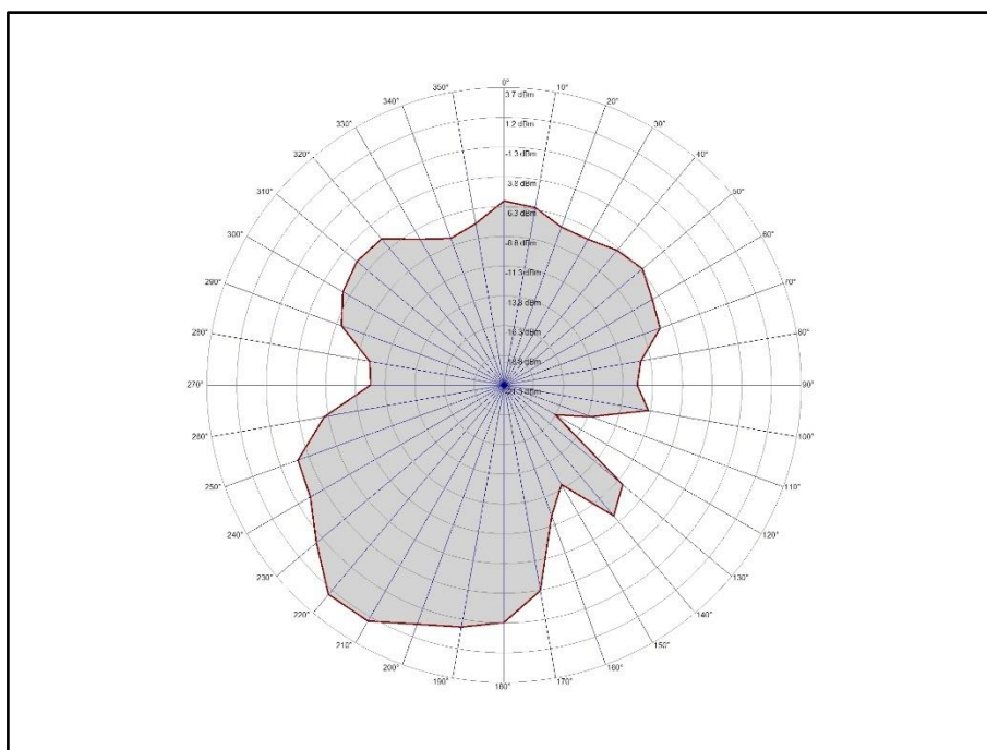
Figure 3 - 2402 MHz, Horizontal
