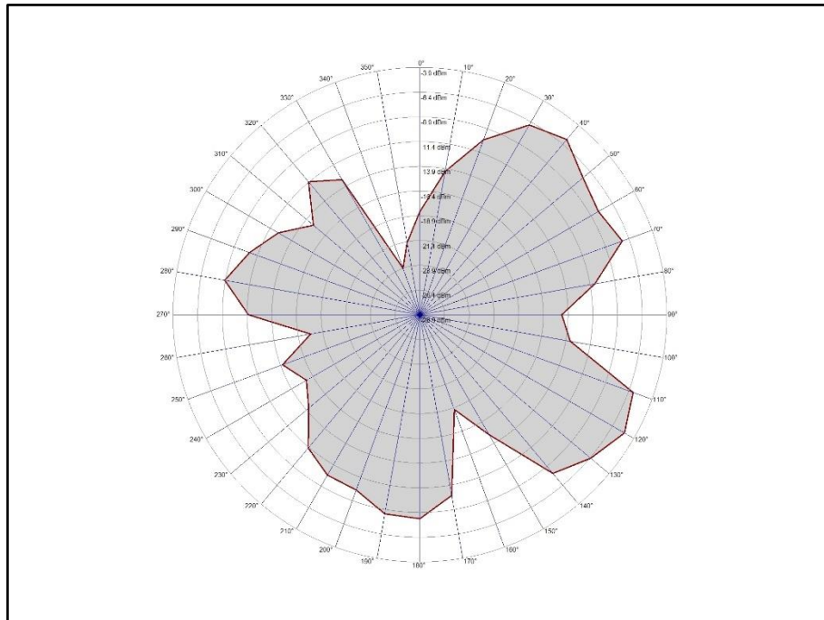
Figure 4 - 2402 MHz, Vertical
