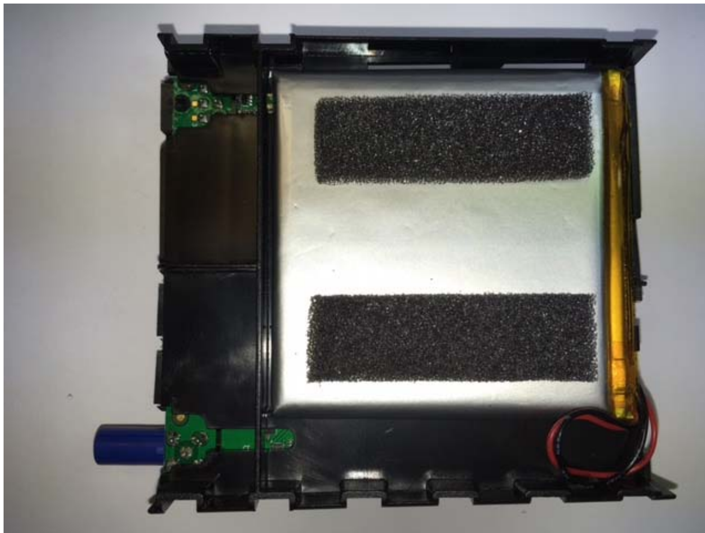
Figure 4- View of Underside of Main Board and Battery Fitted to Carrier
