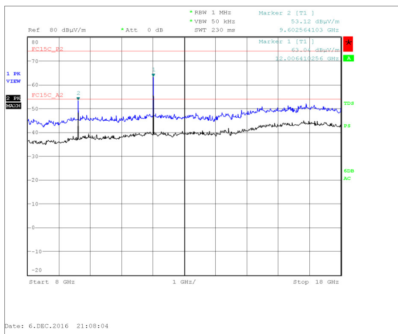
Figure 7 - Frequency Range Under Test: 8 GHz to 18 GHz - Polarity: Horizontal and Vertical
