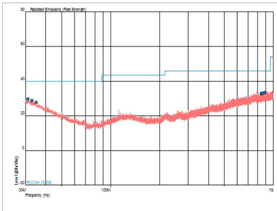
Figure 9 - Frequency Range Under Test: 30 MHz to 1 GHz - Polarity Horizontal and Vertical
