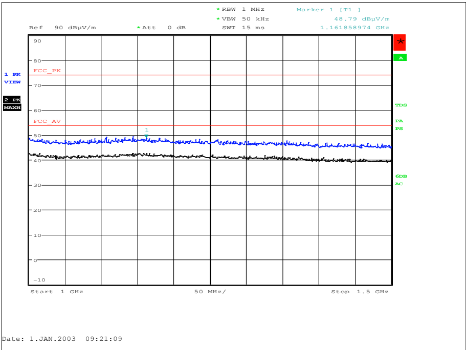
Figure 32 - 915 MHz - 1 GHz to 1.5 GHz - Z Orientation - Horizontal and Vertical
