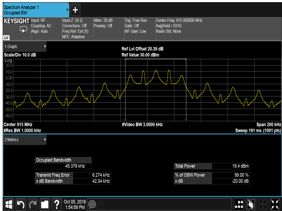
Figure 3 - 915 MHz
