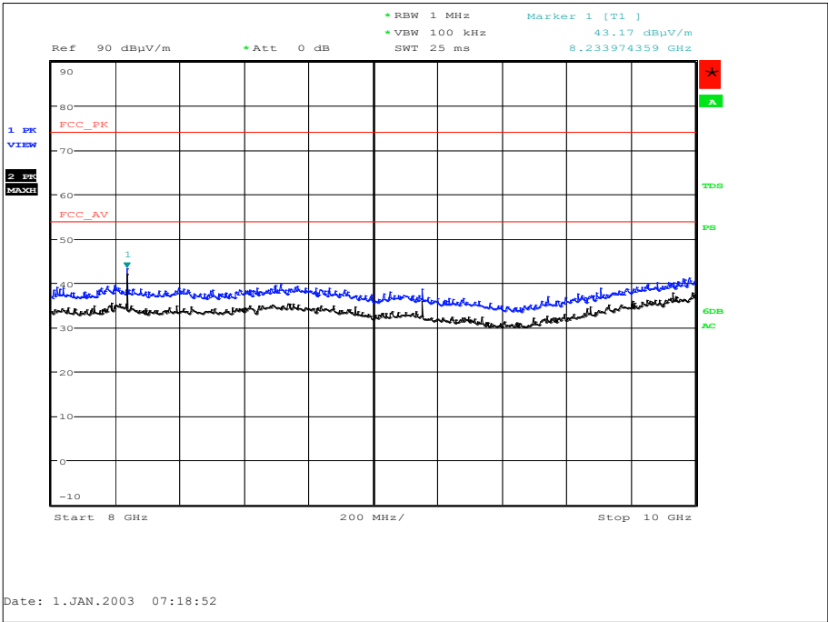
Figure 31 - 915 MHz - 8 GHz to 10 GHz - Y Orientation - Horizontal and Vertical
