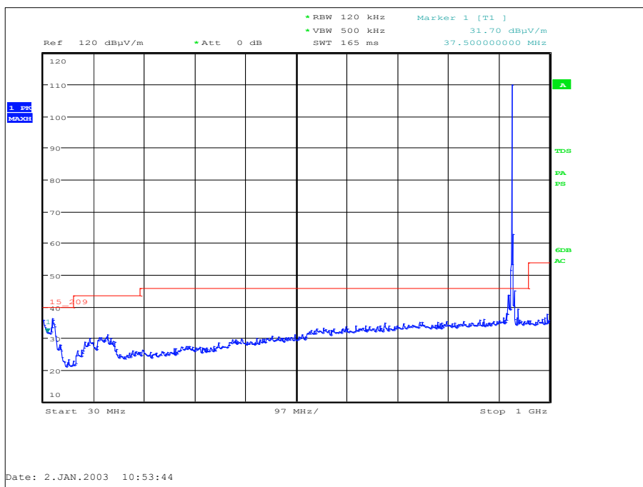
Figure 36 - 927.4 MHz - 30 MHz to 1 GHz - Y Orientation - Horizontal and Vertical
