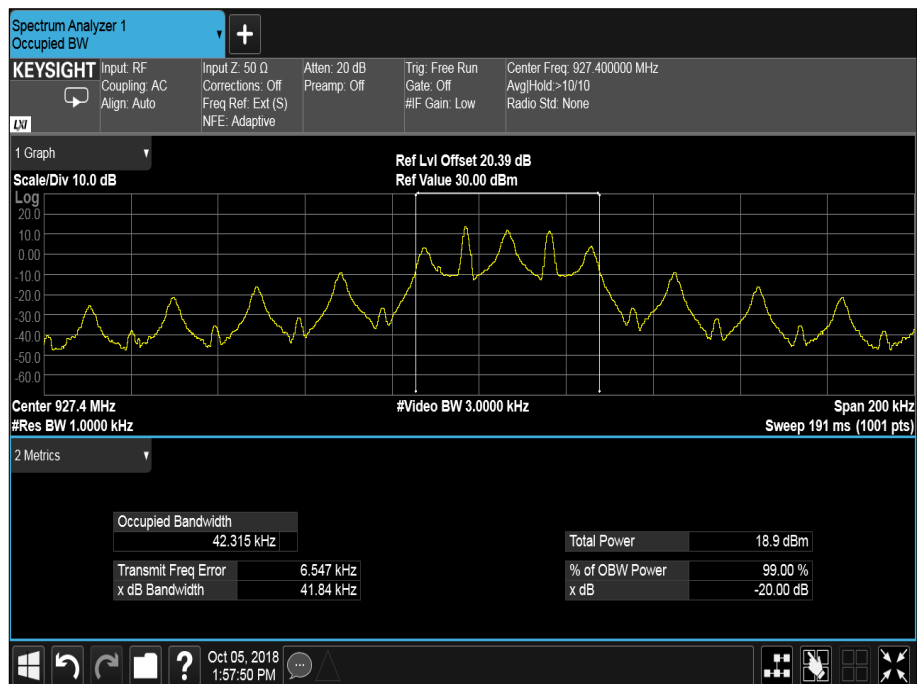
Figure 4 - 927.4 MHz
