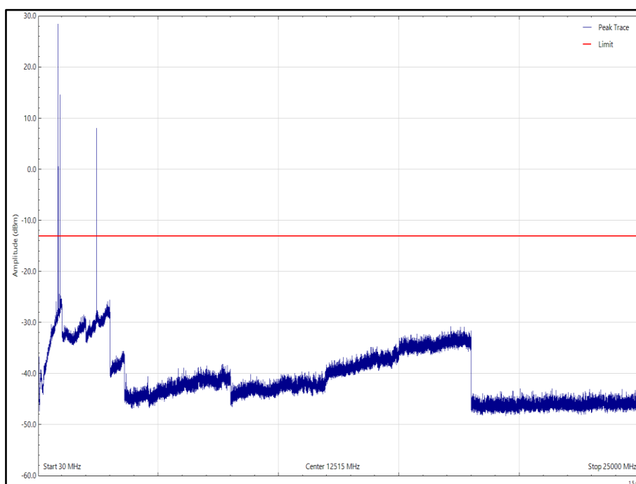
Figure 14 - BLE (2440 MHz), SRD (915 MHz) & LTE FDD Band 5 (836.5 MHz), Orientation: X, 30 MHz to 25 GHz, Horizontal (Peak)
