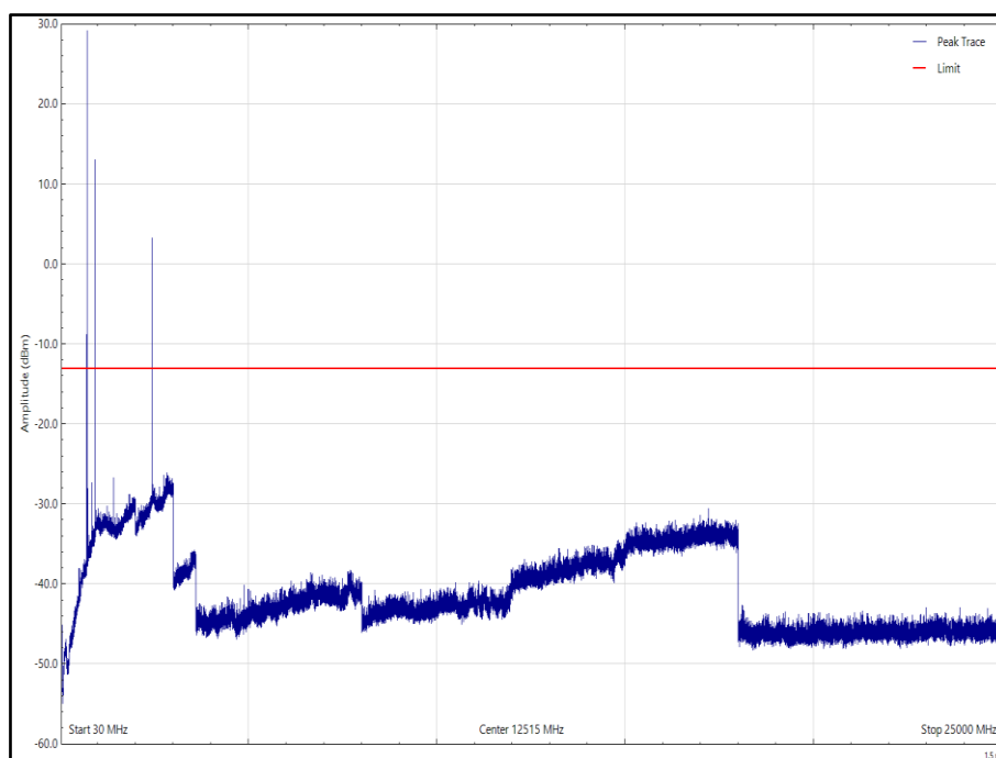
Figure 22 - BLE (2440 MHz), SRD (915 MHz) & LTE FDD Band 12 (707.5 MHz), Orientation: Y, 30 MHz to 25 GHz, Horizontal (Peak)
