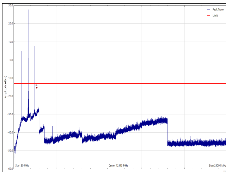
Figure 8- BLE (2440 MHz), SRD (915 MHz) & LTE FDD Band 4 (1732.5 MHz), Orientation: X, 30 MHz to 25 GHz, Horizontal (Peak)
