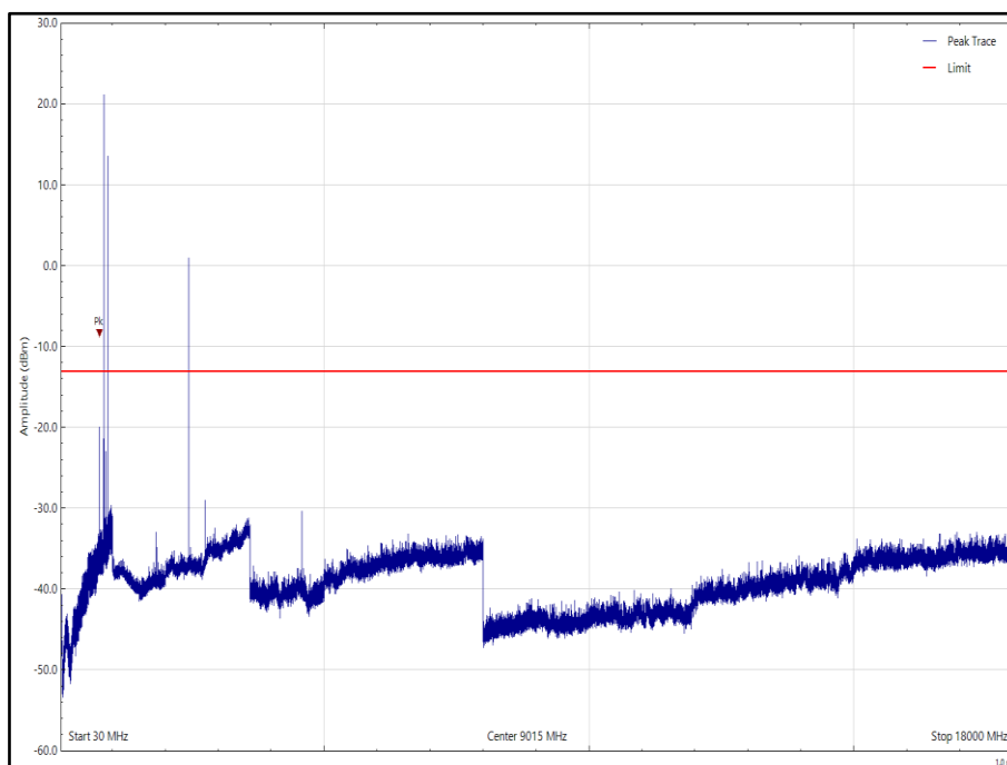
Figure 41 - BLE (2440 MHz), SRD (915 MHz) & LTE-B5 (836.5 MHz) - Y - Orientation, 30 MHz to 18 GHz, Horizontal (Peak)
