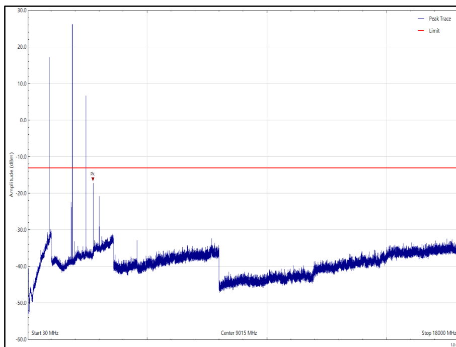
Figure 27 - BLE (2440 MHz), SRD (915 MHz) & PCS 1900 (1880 MHz) - X - Orientation, 30 MHz to 18 GHz, Horizontal (Peak)
