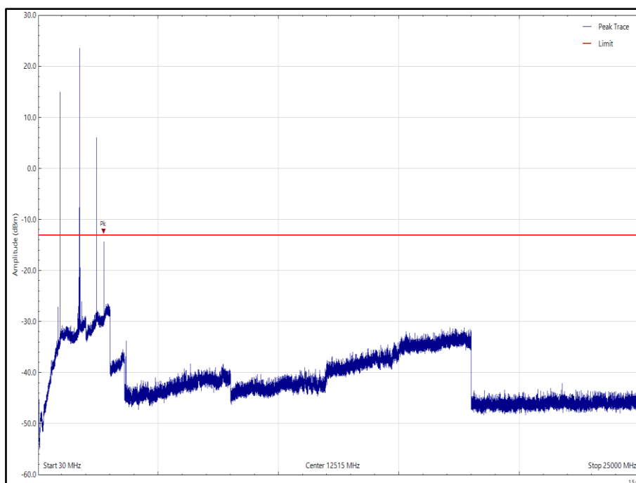
Figure 12 - BLE (2440 MHz), SRD (915 MHz) & LTE FDD Band 4 (1732.5 MHz), Orientation: Z, 30 MHz to 25 GHz, Horizontal (Peak)
