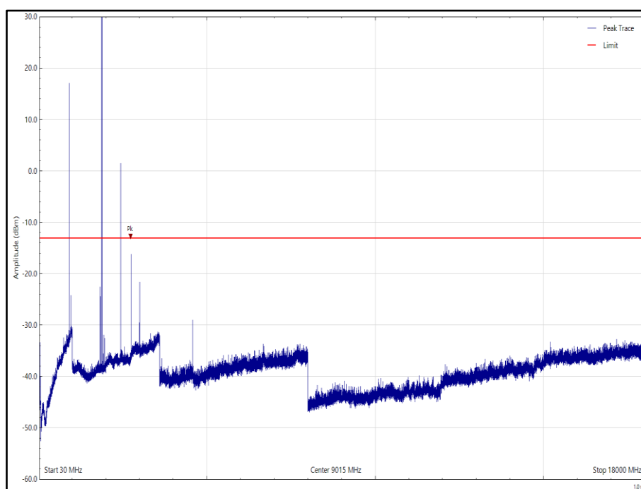
Figure 29 - BLE (2440 MHz), SRD (915 MHz) & PCS 1900 (1880 MHz) - Y - Orientation, 30 MHz to 18 GHz, Horizontal (Peak)
