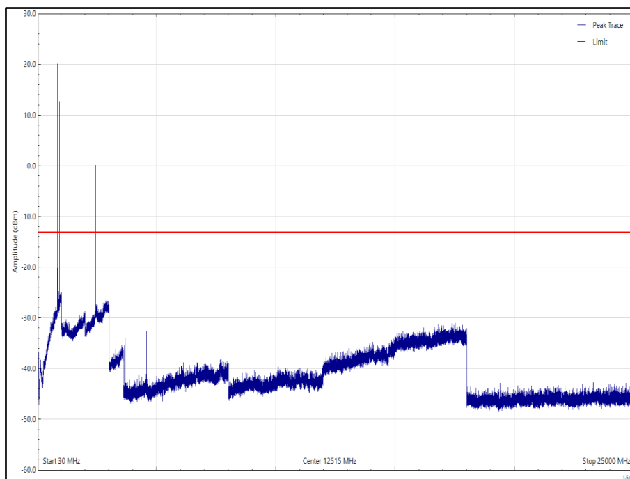
Figure 16 - BLE (2440 MHz), SRD (915 MHz) & LTE FDD Band 5 (836.5 MHz), Orientation: Y, 30 MHz to 25 GHz, Horizontal (Peak)
