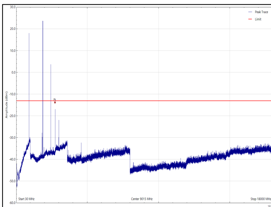
Figure 31 - BLE (2440 MHz), SRD (915 MHz) & PCS 1900 (1880 MHz) - X - Orientation, 30 MHz to 18 GHz, Horizontal (Peak)
