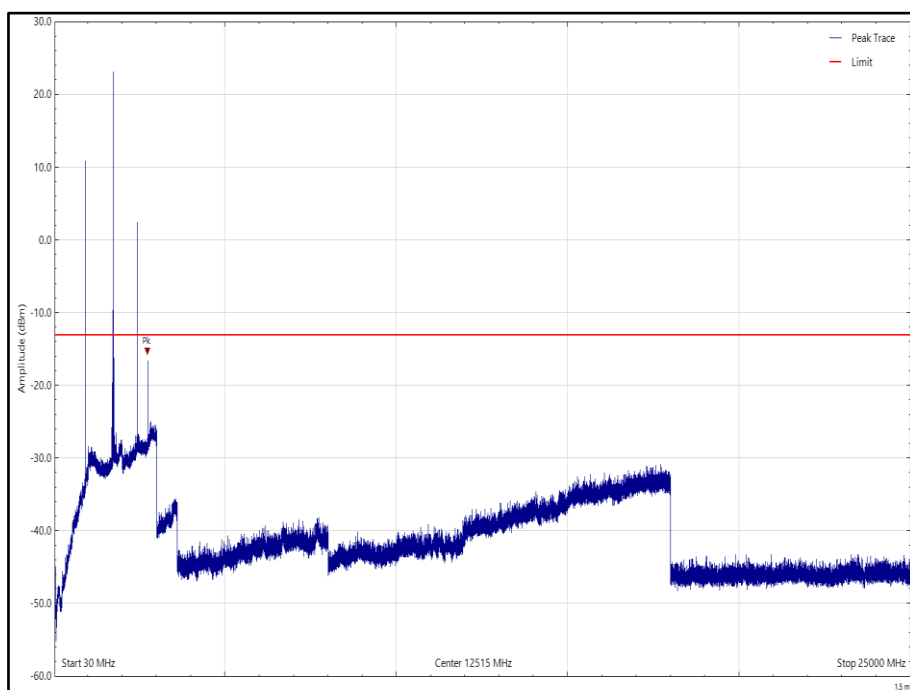
Figure 9 - BLE (2440 MHz), SRD (915 MHz) & LTE FDD Band 4 (1732.5 MHz), Orientation: X, 30 MHz to 25 GHz, Vertical (Peak)
