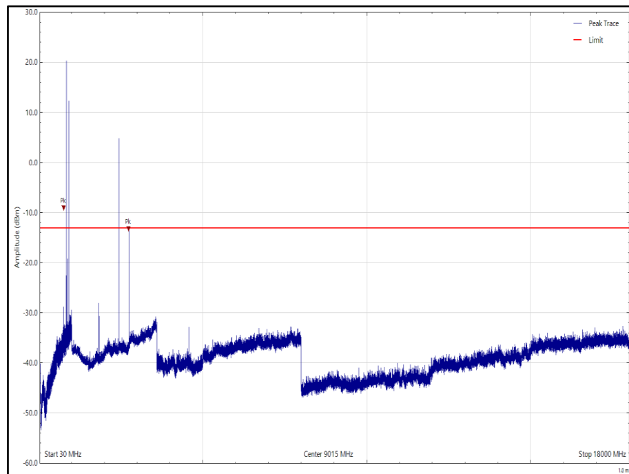
Figure 42 - BLE (2440 MHz), SRD (915 MHz) & LTE-B5 (836.5 MHz) - Y - Orientation, 30 MHz to 18 GHz, Vertical (Peak)
