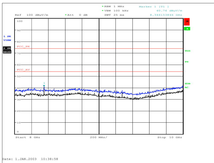
Figure 46 - 927.4 MHz - 8 GHz to 10 GHz - Z Orientation - Horizontal and Vertical
