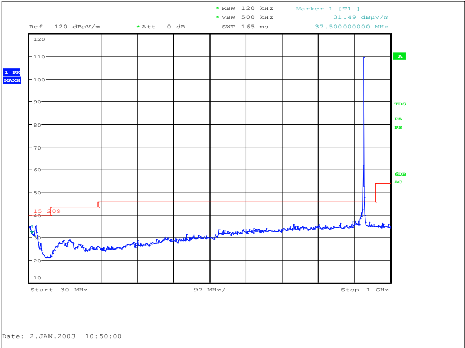
Figure 35 - 927.4 MHz - 30 MHz to 1 GHz - X Orientation - Horizontal and Vertical
