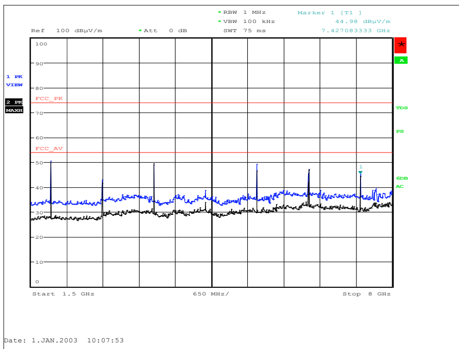
Figure 42 - 927.4 MHz - 1.5 GHz to 8 GHz - Y Orientation - Horizontal and Vertical
