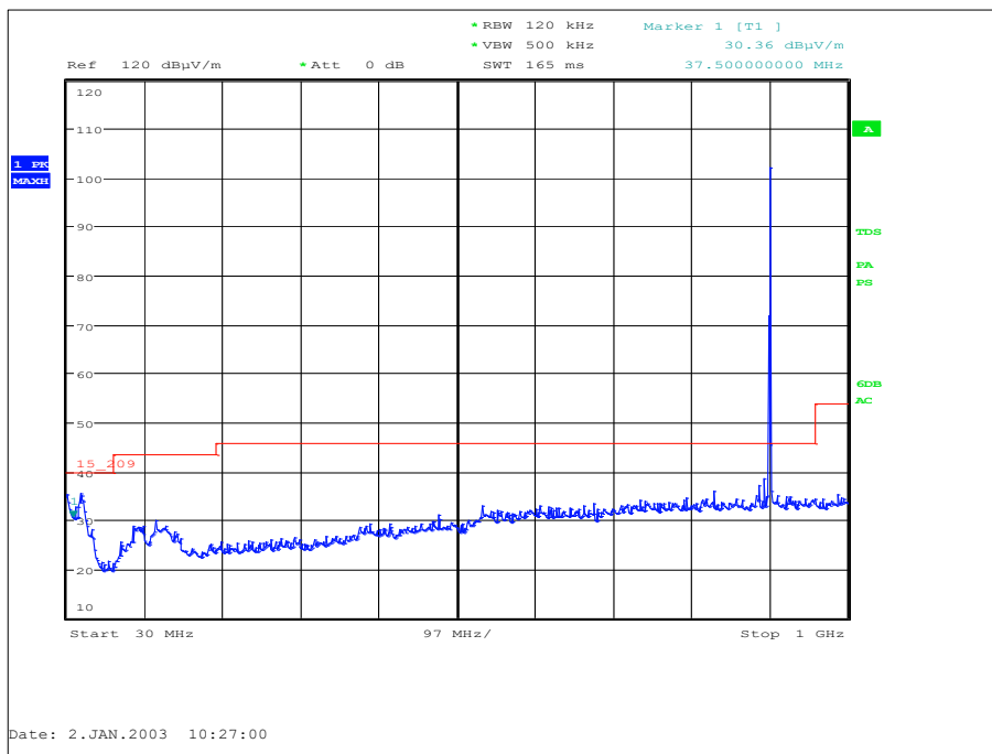
Figure 12 - 902.2 MHz - 30 MHz to 1 GHz - Y Orientation - Horizontal and Vertical
