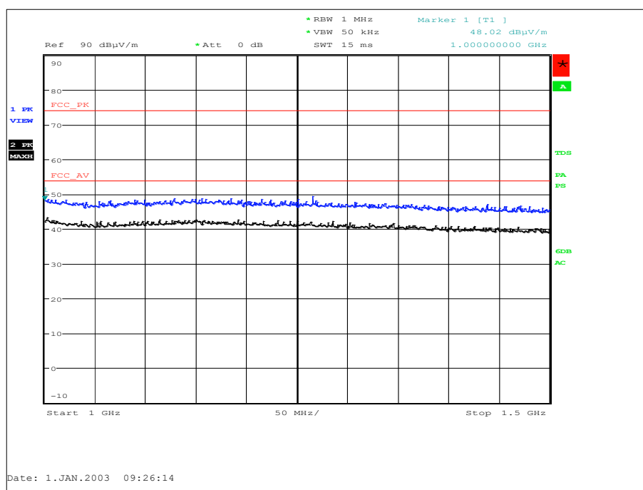
Figure 44 - 927.4 MHz - 1 GHz to 1.5 GHz - Z Orientation - Horizontal and Vertical
