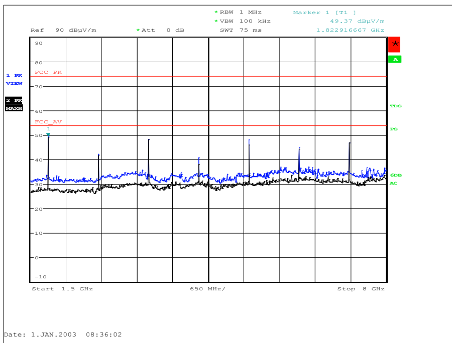
Figure 30 - 915 MHz - 1.5 GHz to 8 GHz - Y Orientation - Horizontal and Vertical
