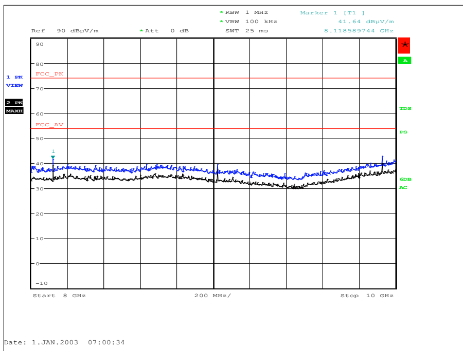
Figure 22 - 902.2 MHz - 8 GHz to 10 GHz - Z Orientation - Horizontal and Vertical
