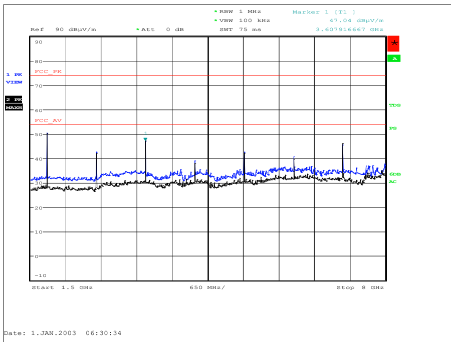
Figure 21 - 902.2 MHz - 1.5 GHz to 8 GHz - Z Orientation - Horizontal and Vertical
