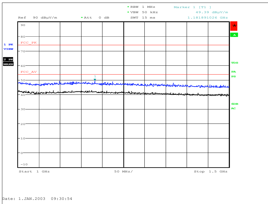
Figure 41 - 927.4 MHz - 1 GHz to 1.5 GHz - Y Orientation - Horizontal and Vertical
