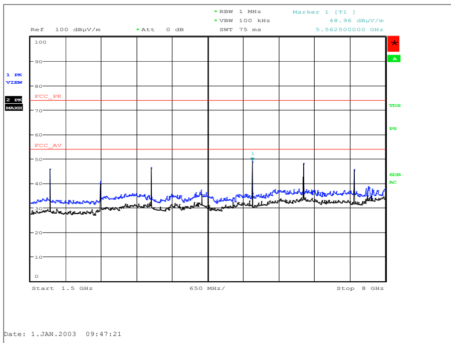
Figure 39 - 927.4 MHz - 1.5 GHz to 8 GHz - X Orientation - Horizontal and Vertical
