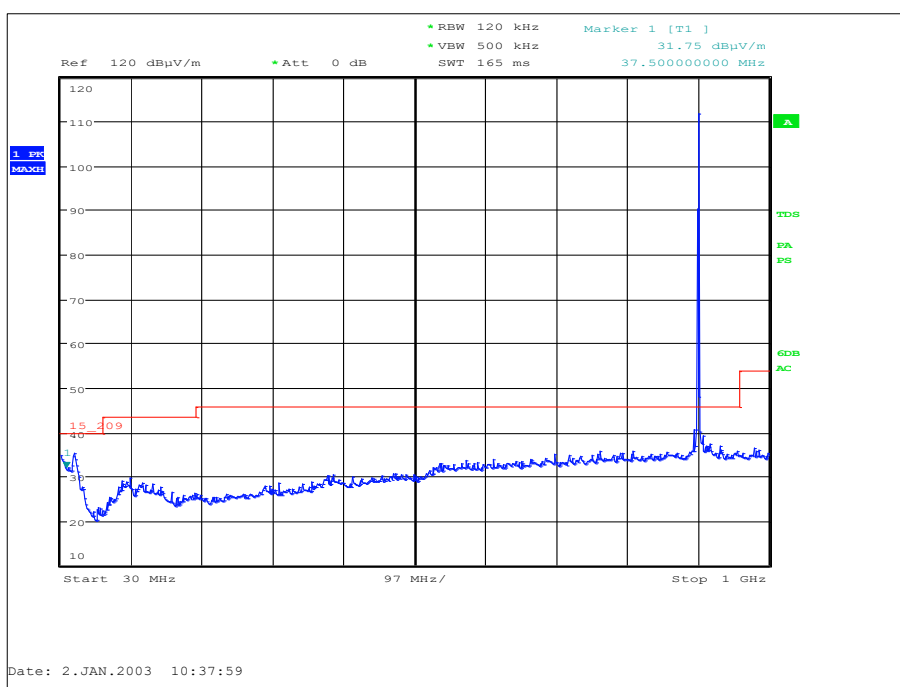
Figure 11 - 902.2 MHz - 30 MHz to 1 GHz - X Orientation - Horizontal and Vertical
