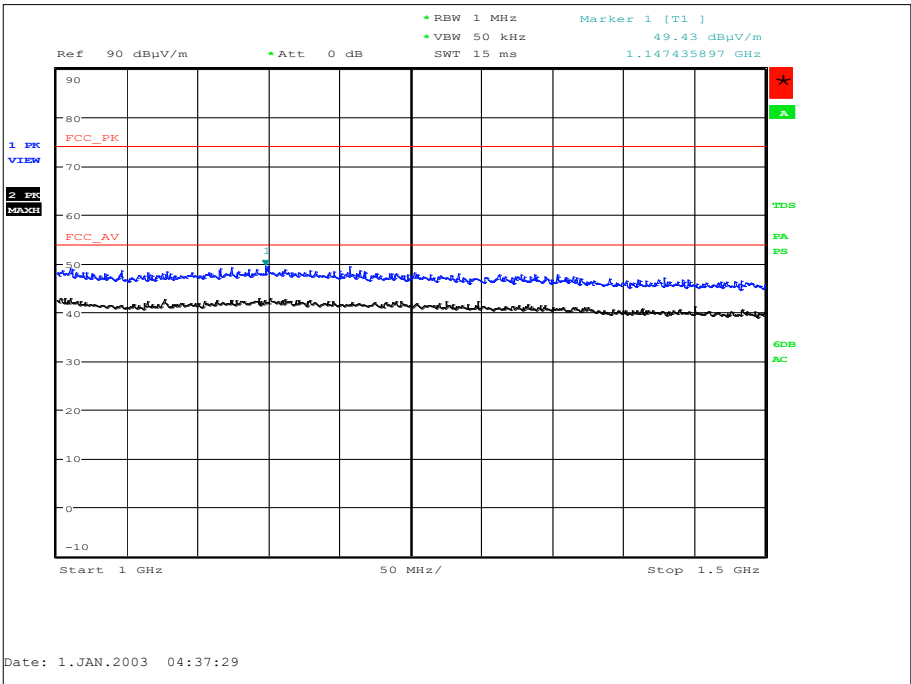
Figure 14 - 902.2 MHz - 1 GHz to 1.5 GHz - X Orientation - Horizontal and Vertical
