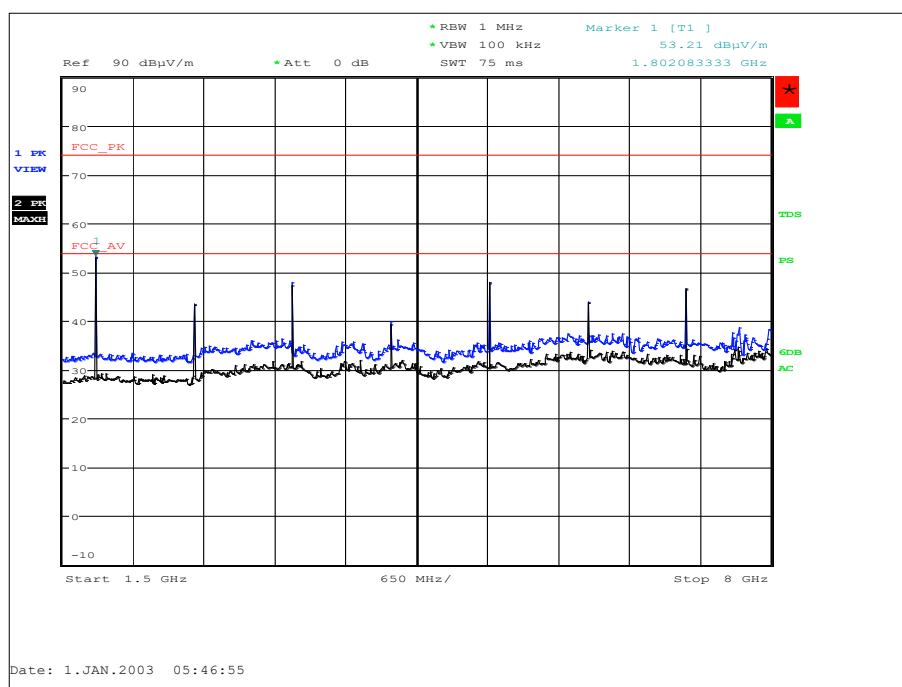
Figure 18 - 902.2 MHz - 1.5 GHz to 8 GHz - Y Orientation - Horizontal and Vertical
