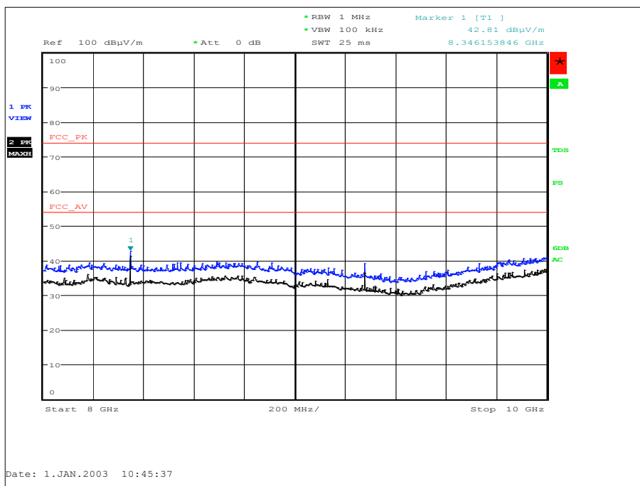
Figure 40 - 927.4 MHz - 8 GHz to 10 GHz - X Orientation - Horizontal and Vertical
