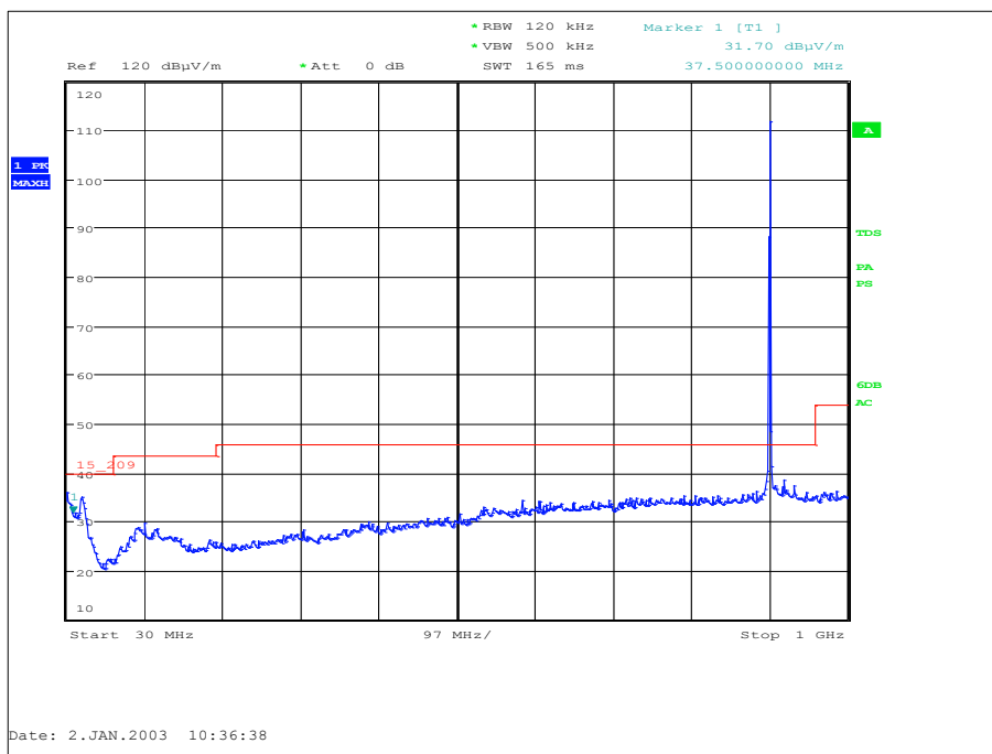
Figure 13 - 902.2 MHz - 30 MHz to 1 GHz - Z Orientation - Horizontal and Vertical
