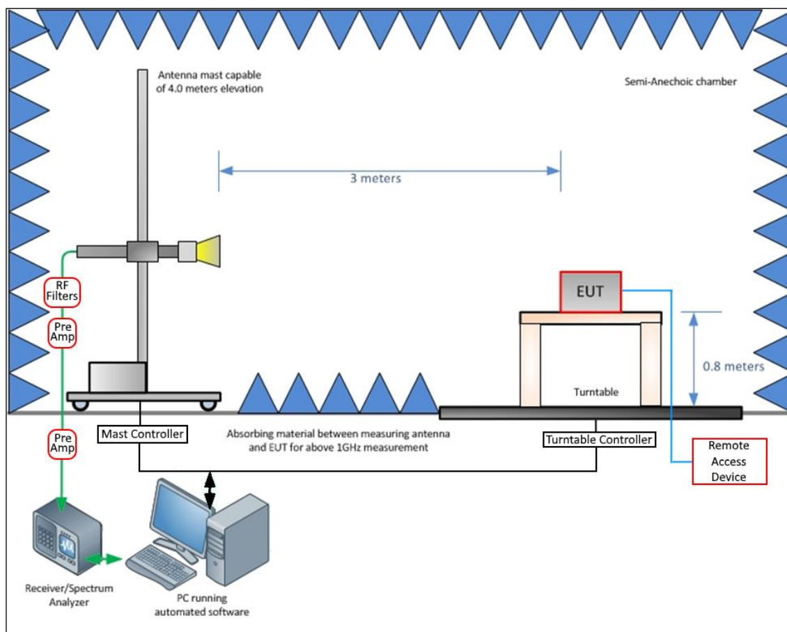
Figure 1 - Radiated Disturbance Example Test Setup
