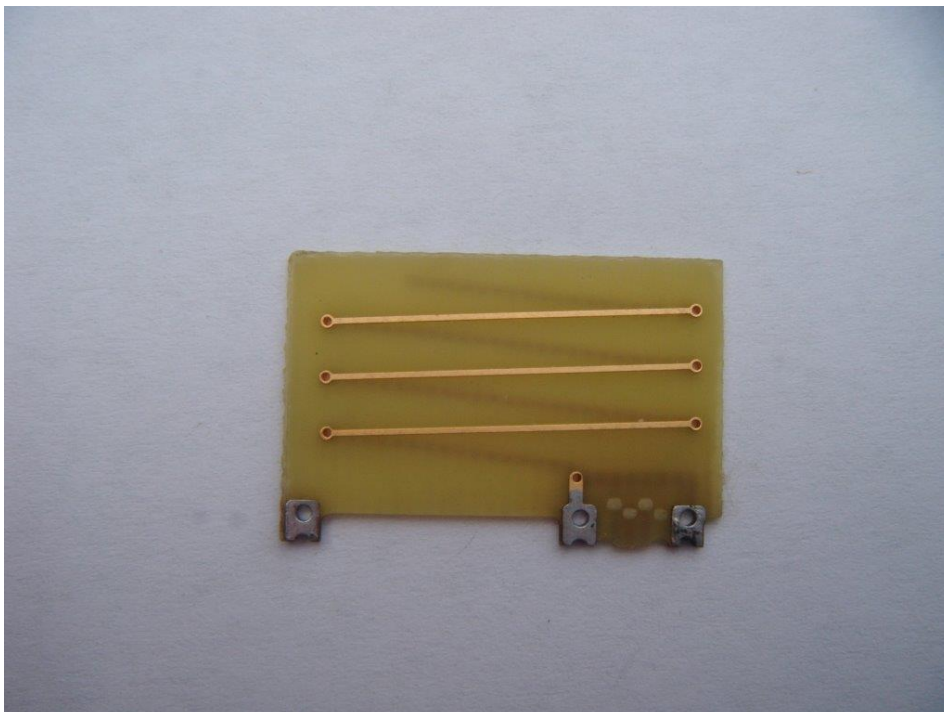
View of antenna pcb – bottom side
