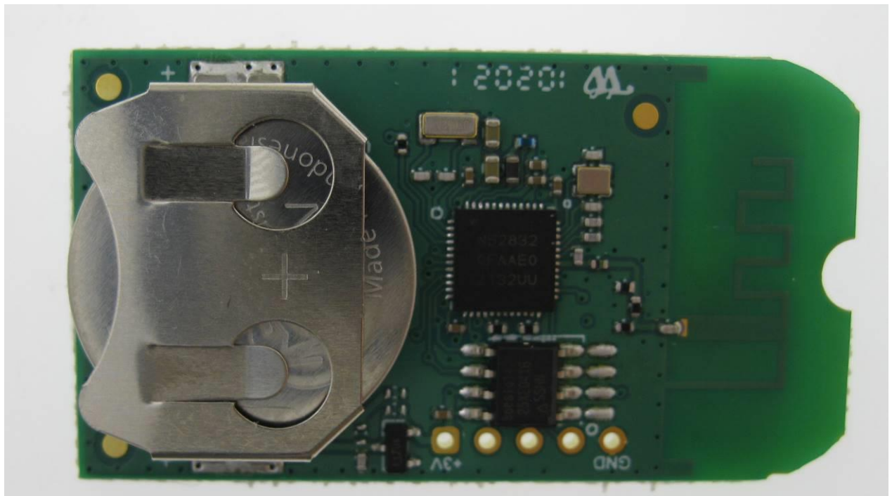
BT HOS DID – PCB front
