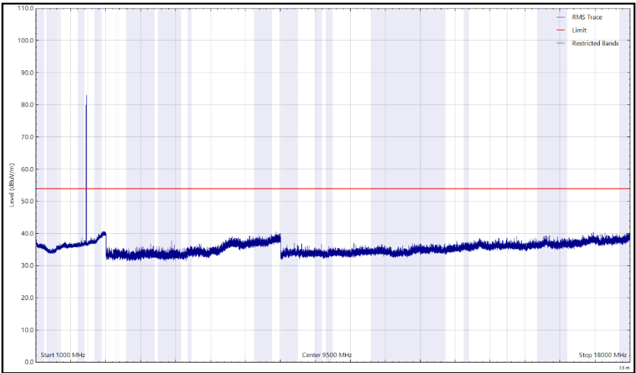
Figure 38 - 2440 MHz (CH17), LE1M – Y Orientation, 1 GHz to 18 GHz, Horizontal (rms)
