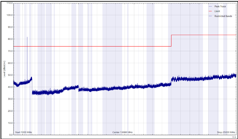
Figure 28 - 2480 MHz (CH39), LE1M – X Orientation, 1 GHz to 25 GHz, Vertical (Peak)
