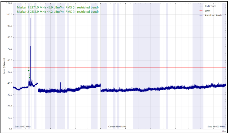
Figure 50 - 2402 MHz (CH37), LE1M – Z Orientation, 1 GHz to 18 GHz, Horizontal (rms)
