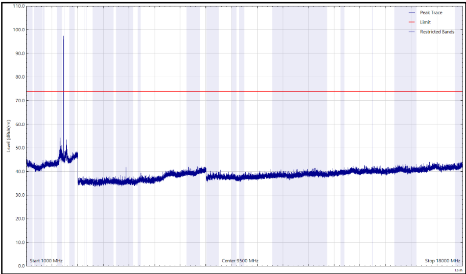
Figure 40 - 2440 MHz (CH17), LE1M – Y Orientation, 1 GHz to 18 GHz, Vertical (Peak)
