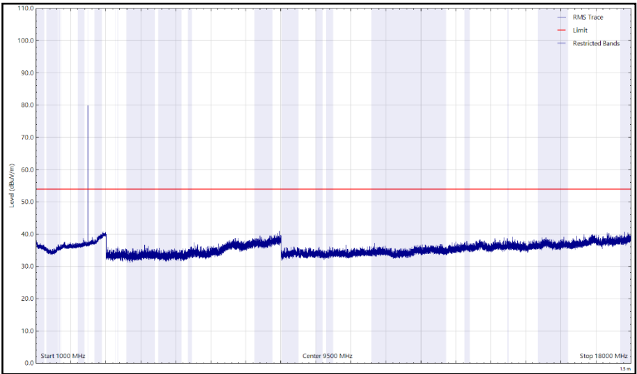
Figure 44 - 2480 MHz (CH39), LE1M – Y Orientation, 1 GHz to 18 GHz, Horizontal (rms)
