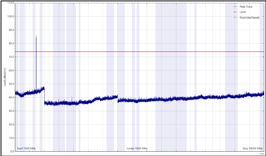
Figure 58 - 2440 MHz (CH17), LE1M – Z Orientation, 1 GHz to 18 GHz, Vertical (Peak)
