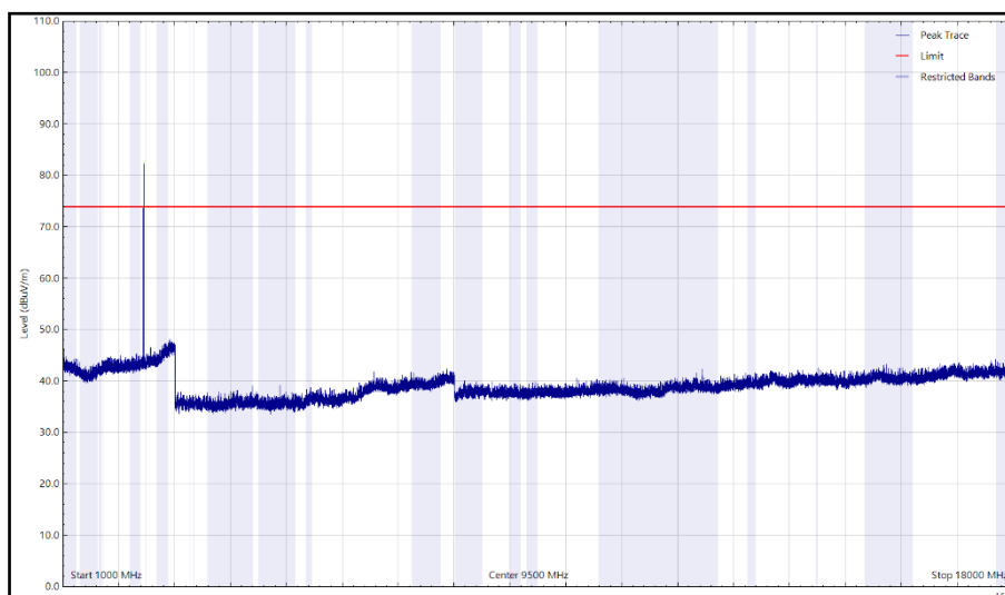
Figure 37 - 2440 MHz (CH17), LE1M – Y Orientation, 1 GHz to 18 GHz, Horizontal (Peak)
