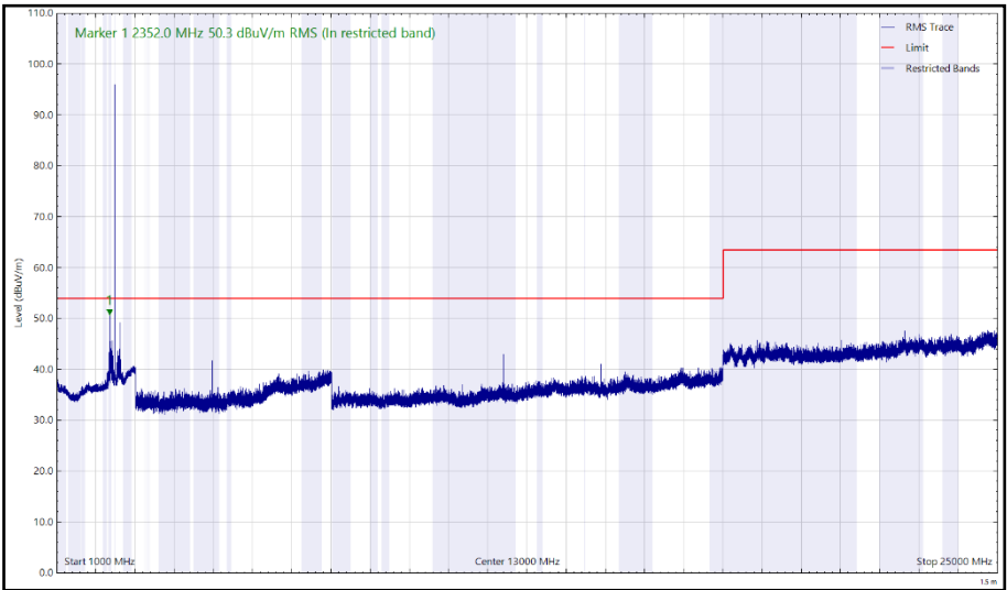
Figure 26 - 2480 MHz (CH39), LE1M – X Orientation, 1 GHz to 25 GHz, Horizontal (rms)
