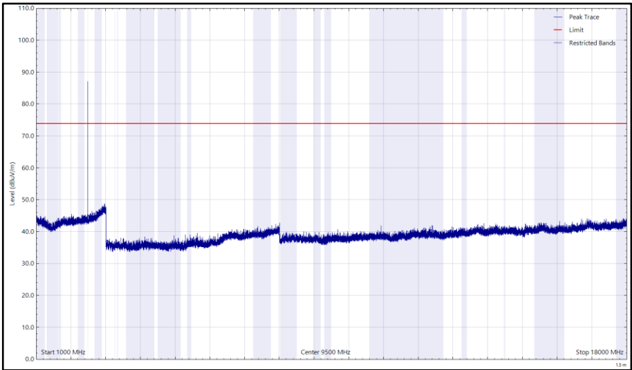
Figure 64 - 2480 MHz (CH39), LE1M – Z Orientation, 1 GHz to 18 GHz, Vertical (Peak)
