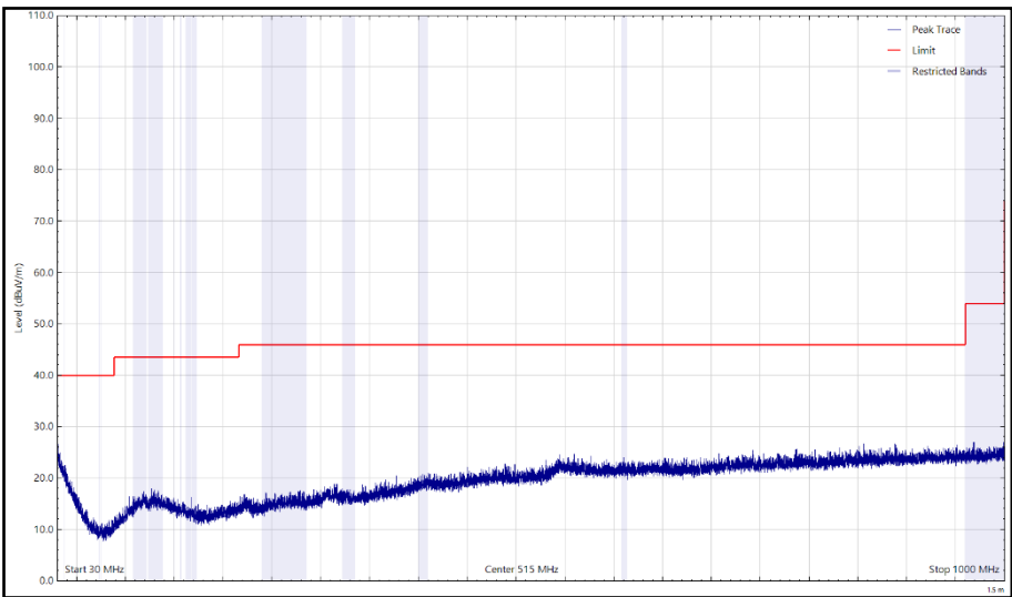
Figure 12 - 2402 MHz (CH37), LE1M – X Orientation, 30 MHz to 1 GHz, Horizontal (Peak)
