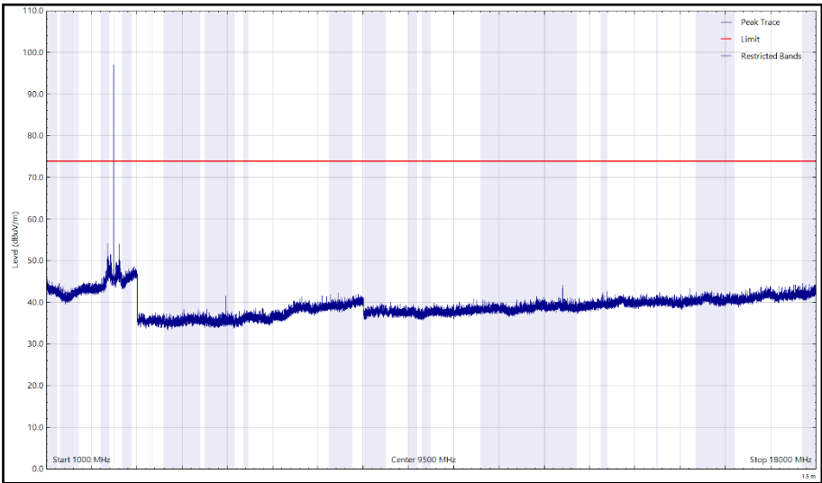
Figure 46 - 2480 MHz (CH39), LE1M – Y Orientation, 1 GHz to 18 GHz, Vertical (Peak)
