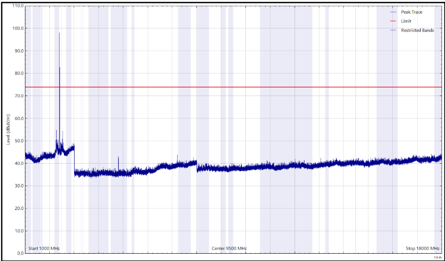
Figure 34 - 2402 MHz (CH37), LE1M – Y Orientation, 1 GHz to 18 GHz, Vertical (Peak)
