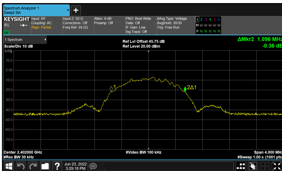
Figure 3 - A (A) 2402 MHz (CH37) 99% Bandwidth
