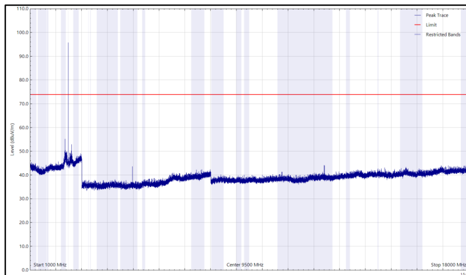
Figure 61 - 2480 MHz (CH39), LE1M – Z Orientation, 1 GHz to 18 GHz, Horizontal (Peak)
