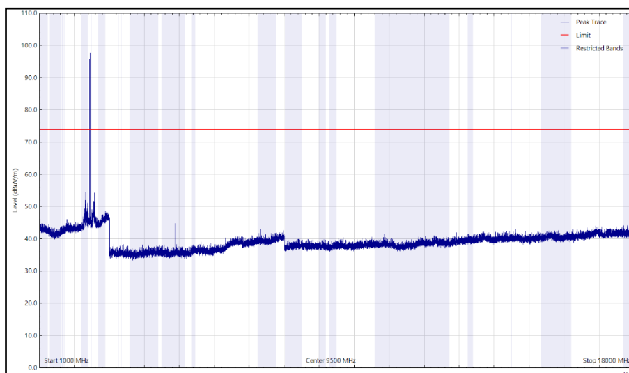
Figure 55 - 2440 MHz (CH17), LE1M – Z Orientation, 1 GHz to 18 GHz, Horizontal (Peak)
