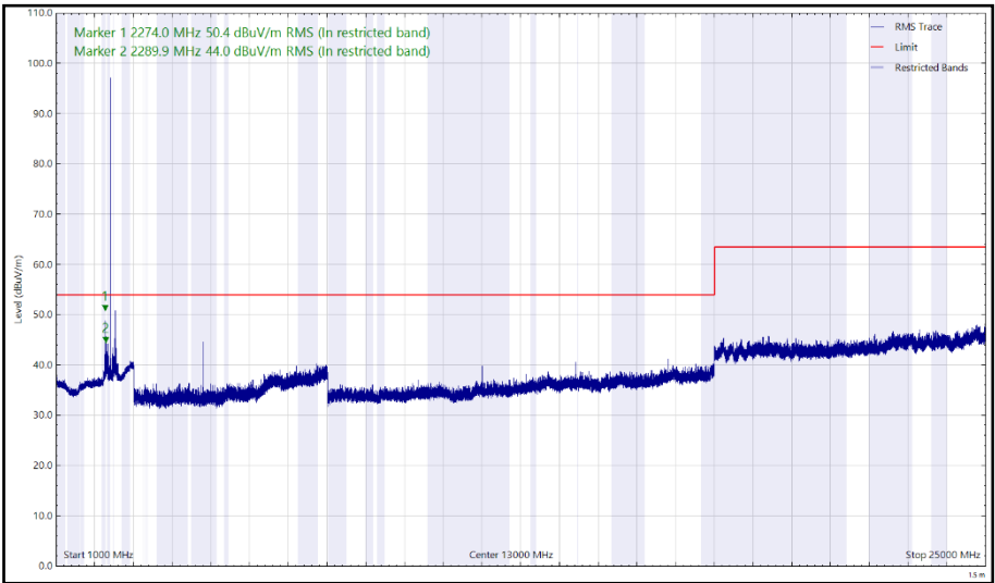
Figure 14 - 2402 MHz (CH37), LE1M, 1 GHz to 25 GHz, Horizontal (rms)
