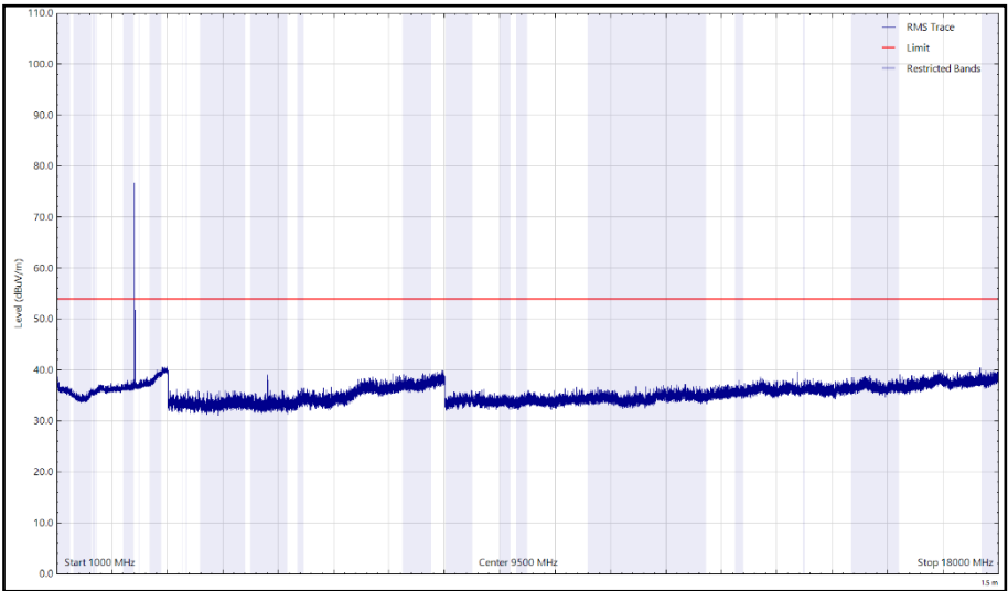
Figure 32 - 2402 MHz (CH37), LE1M – Y Orientation, 1 GHz to 18 GHz, Horizontal (rms)
