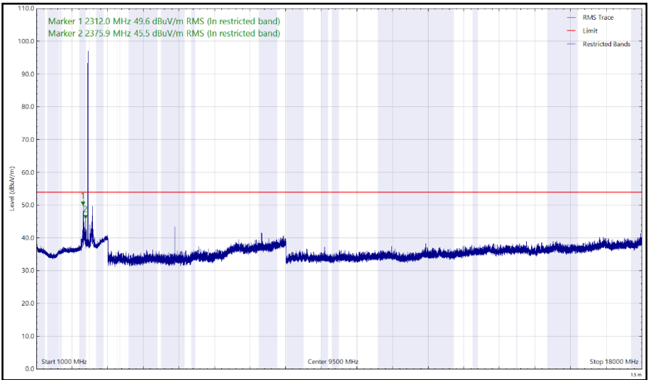
Figure 56 - 2440 MHz (CH17), LE1M – Z Orientation, 1 GHz to 18 GHz, Horizontal (rms)
