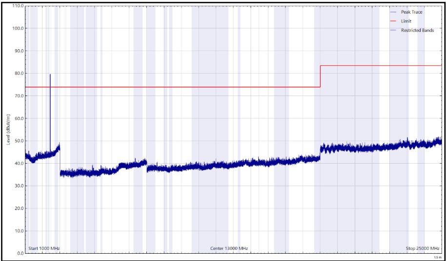
Figure 22 - 2440 MHz (CH17), LE1M – X Orientation, 1 GHz to 25 GHz, Vertical (Peak)
