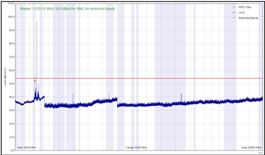
Figure 62 - 2480 MHz (CH39), LE1M – Z Orientation, 1 GHz to 18 GHz, Horizontal (rms)
