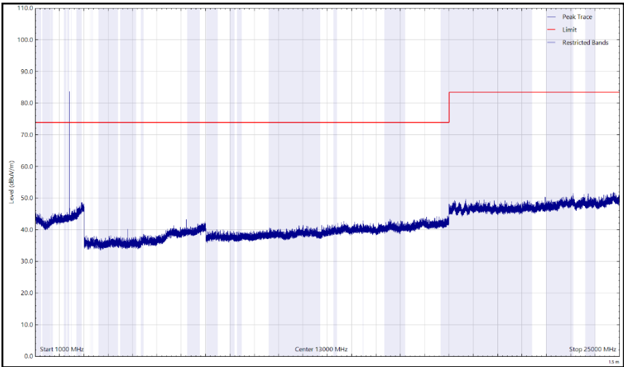
Figure 16 - 2402 MHz (CH37), LE1M – X Orientation, 1 GHz to 25 GHz, Vertical (Peak)
