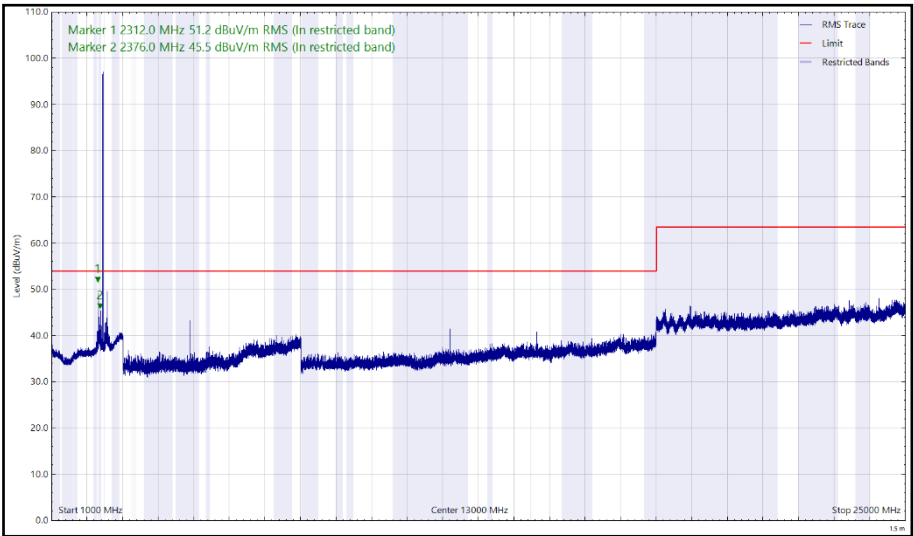
Figure 20 - 2440 MHz (CH17), LE1M – X Orientation, 1 GHz to 25 GHz, Horizontal (rms)
