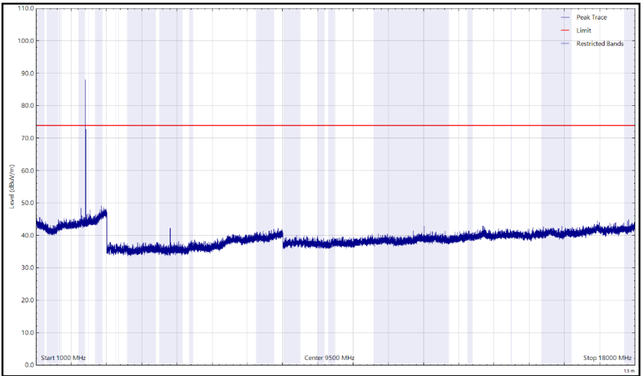
Figure 52 - 2402 MHz (CH37), LE1M – Z Orientation, 1 GHz to 18 GHz, Vertical (Peak)
