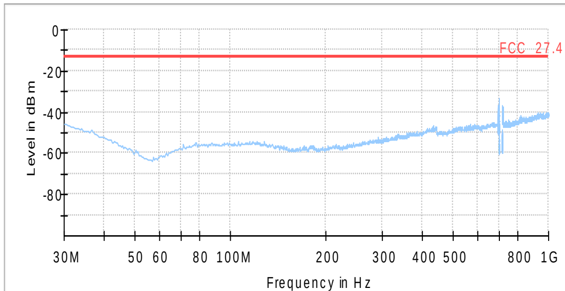
CAT-M1 eFDD12 Channel = mid 30 MHz – 1 GHz
