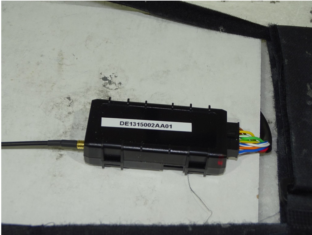
Photo 2: EUT setup
