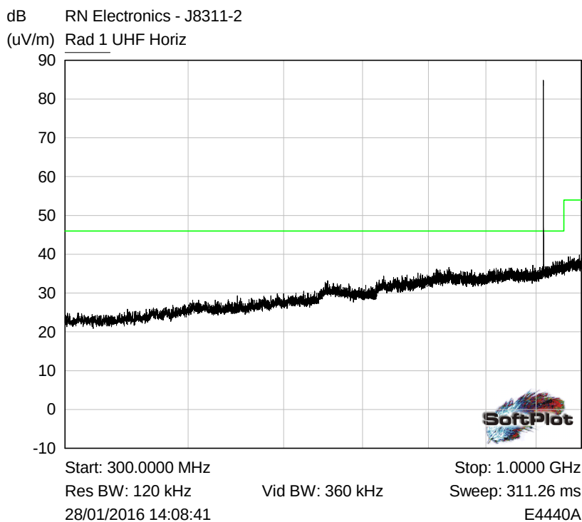
Plot of Peak emissions for UHF Horizontal against the QP limit line. Note: Plot shows the fundamental transmit carrier at 915.18MHz
