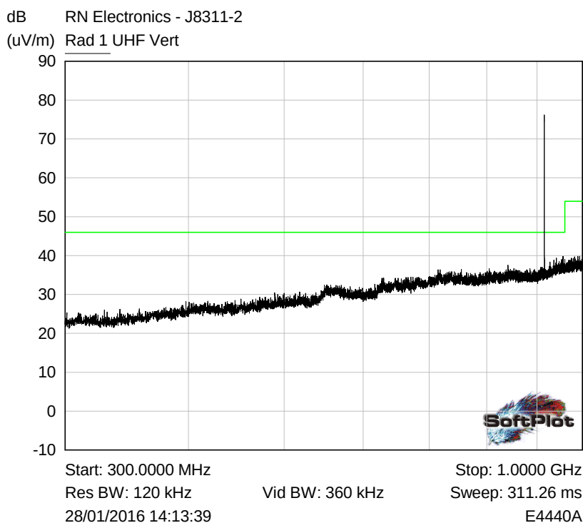
Plot of Peak emissions for UHF Vertical against the QP limit line. Note: Plot shows the fundamental transmit carrier at 915.18MHz
