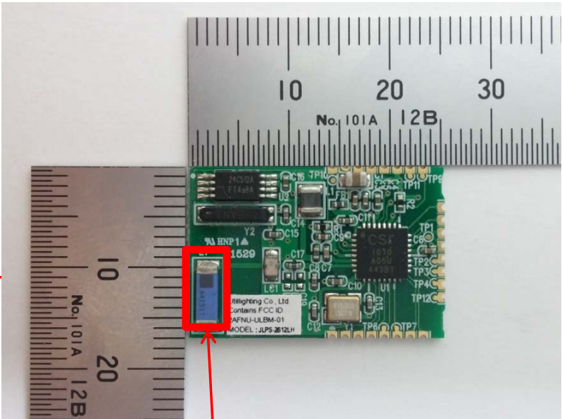
BT ANTENNA
