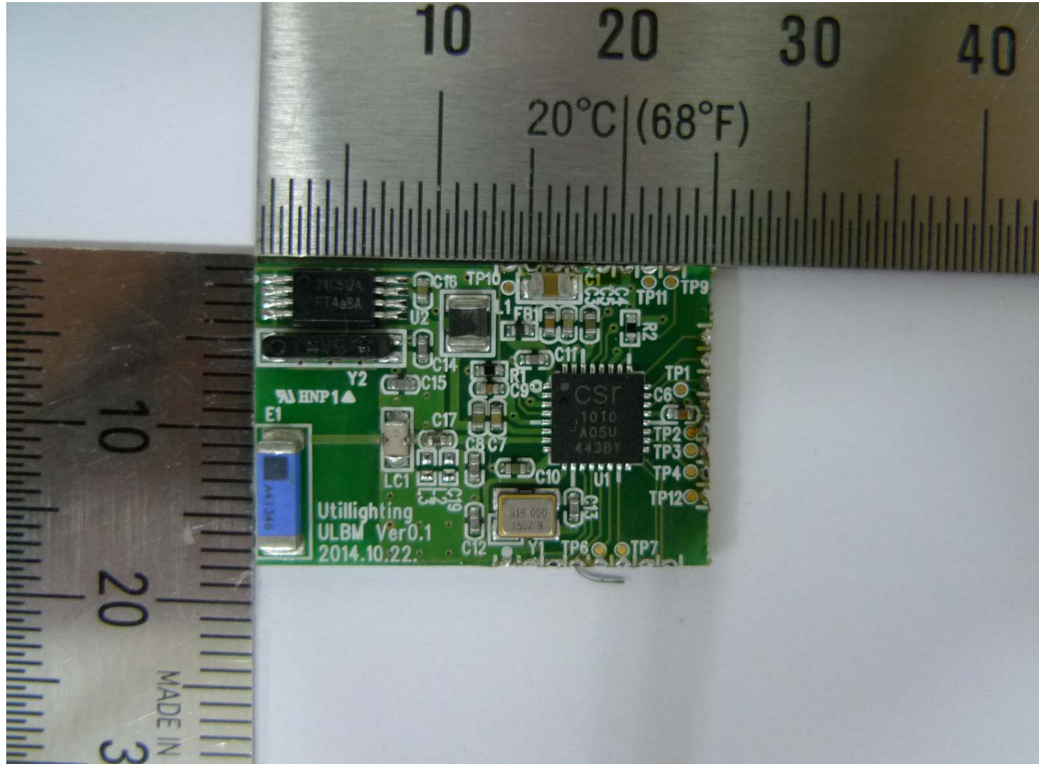
1-1. FRONT
