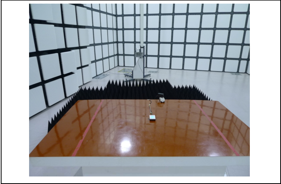
2-2. Setup for Radiated Test (MODEL :JLPS-2612LH) :Above 1 000 MHz [ Front ]
