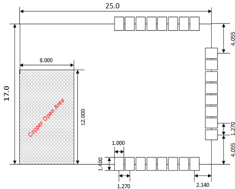
Figure 3-6 Recommended Land Pattern
