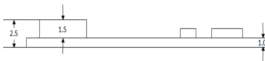
Figure 3-5 Dimension of BLE Module (Side View)
