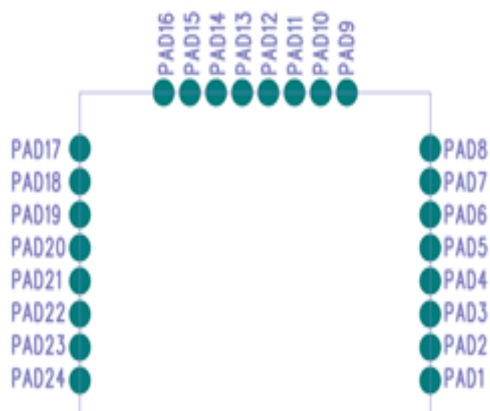
Figure 3-3 Pin out assignment of BLE Module (Top view)
