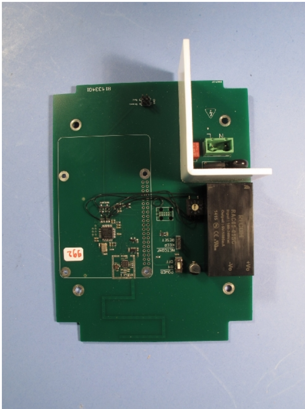
Photograph 5: PCB top view of Router
