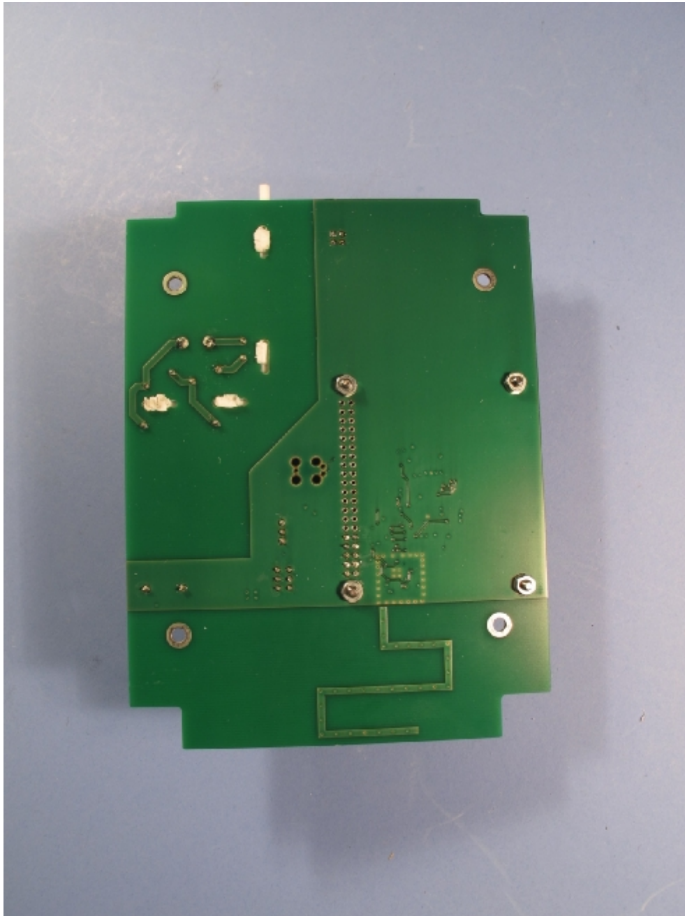
Photograph 3: PCB bottom view of Concentrator
