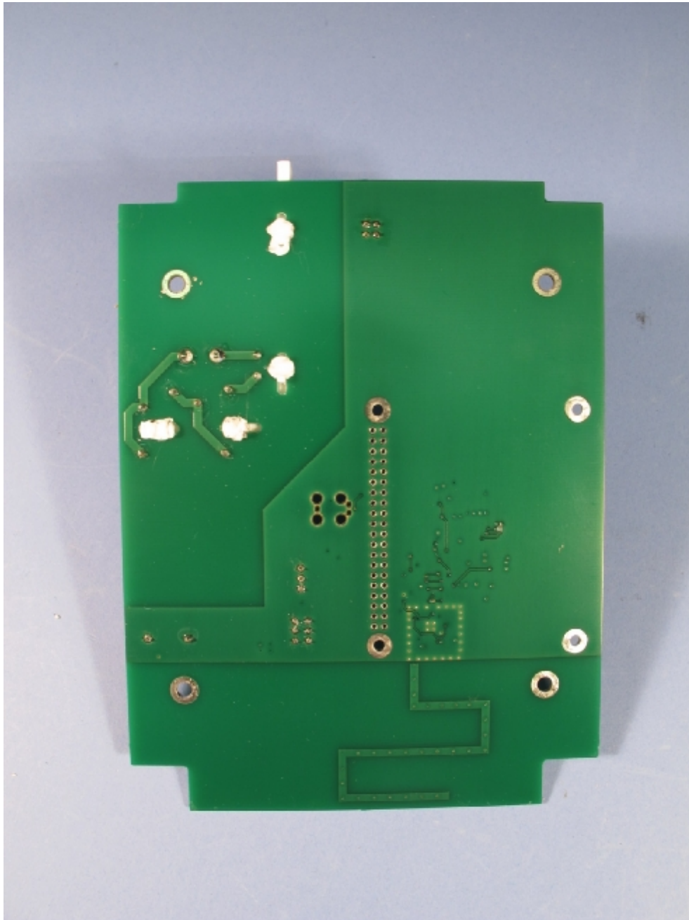
Photograph 6: PCB bottom view of Router
