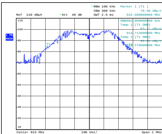
Low channel, 915 MHz
