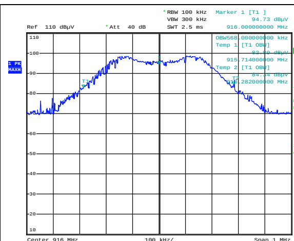
High channel, 916 MHz
