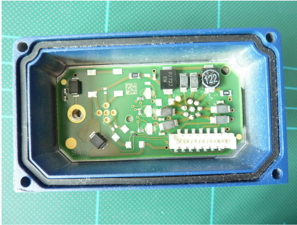
191513EUT14: Sub PCB top view
