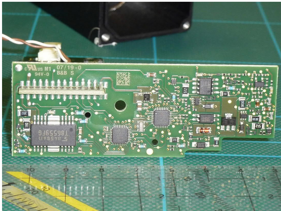
191513EUT1: Main PCBs view 3
