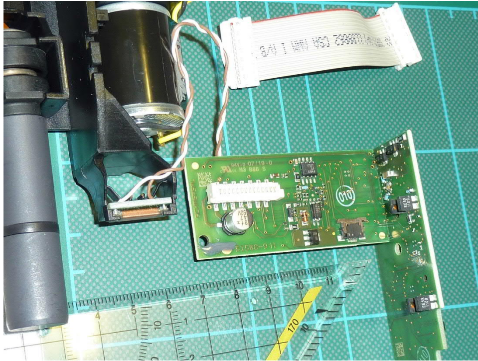
191513EUT08: EUT Inside view 2
