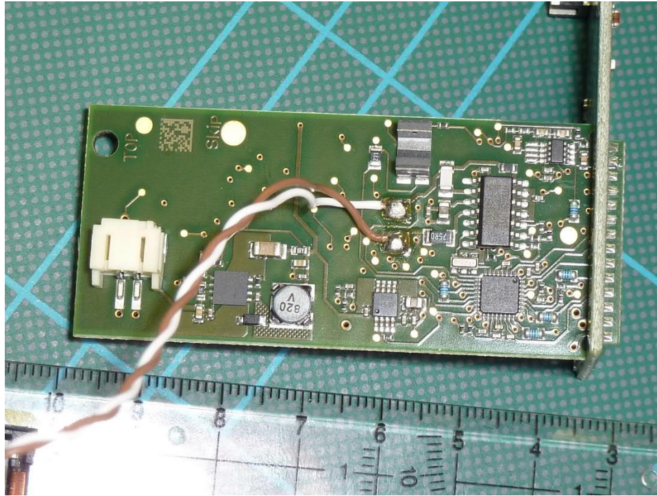
191513EUT10: Main PCBs view 2
