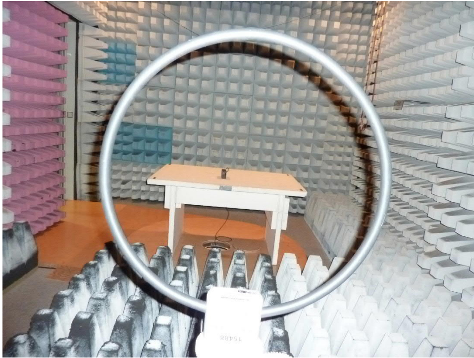
191513_01: Preliminary measurement 9 kHz – 30 MHz
