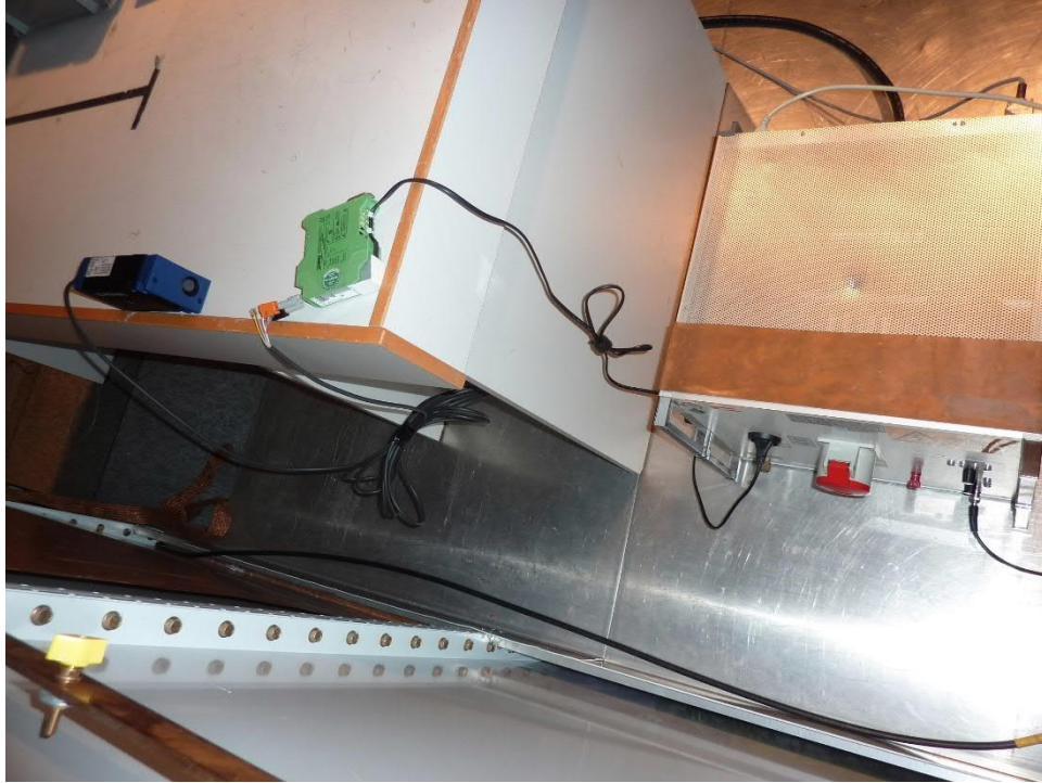
191513_05: Conducted measurement 150 kHz – 30 MHz
