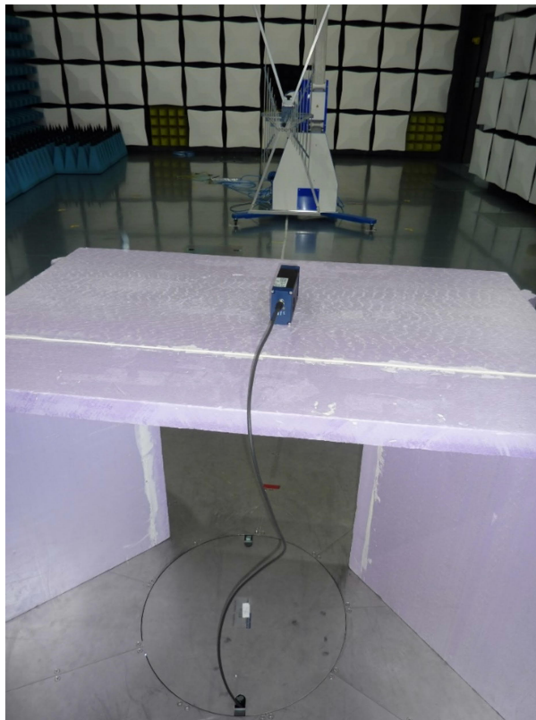
191513_02: Final radiated measurement 30 – 1000 MHz
