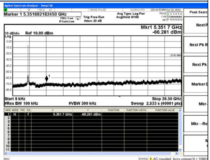
802.11g Chain 0-Middle channel
