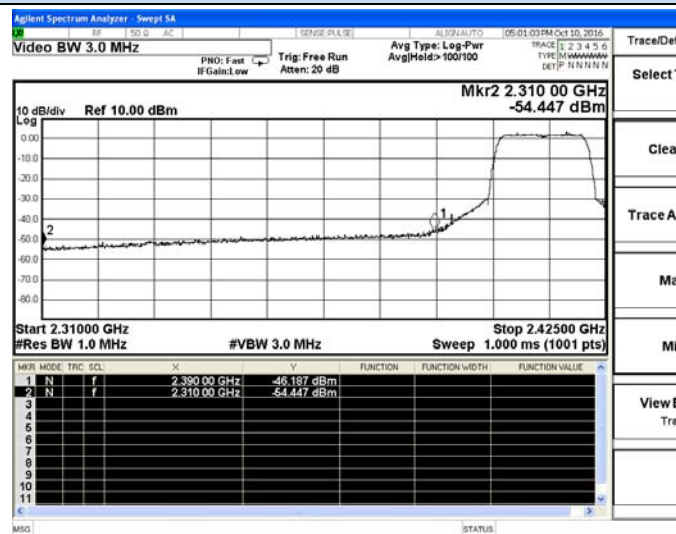
802.11n-HT20 Chain 1-Low channel(Peak)
