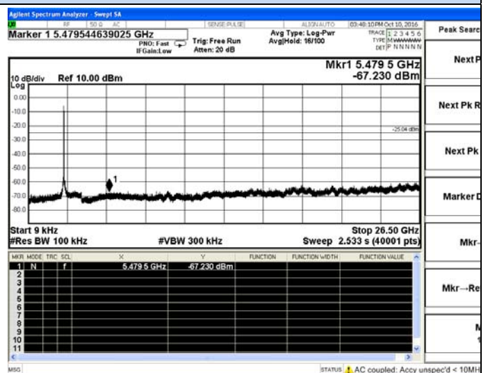
802.11n-HT20 Chain 1-Low channel
