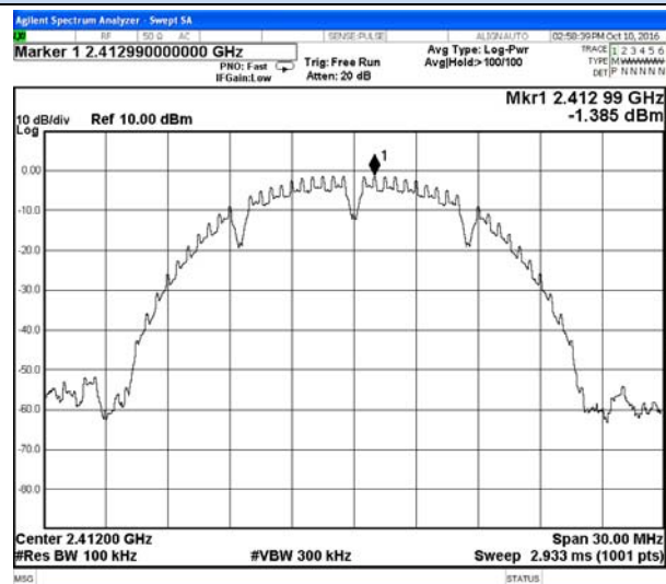
802.11b Chain 0-Low channel Reference
