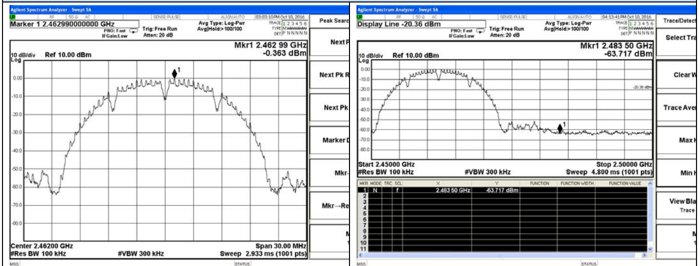
802.11b Chain 1-High channel Reference
