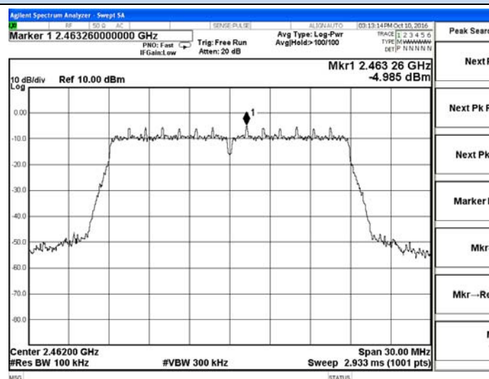
802.11n-HT20 Chain 1-High channel Reference
