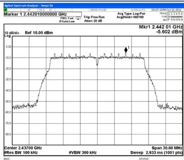
802.11g Chain 0-Middle channel Reference
