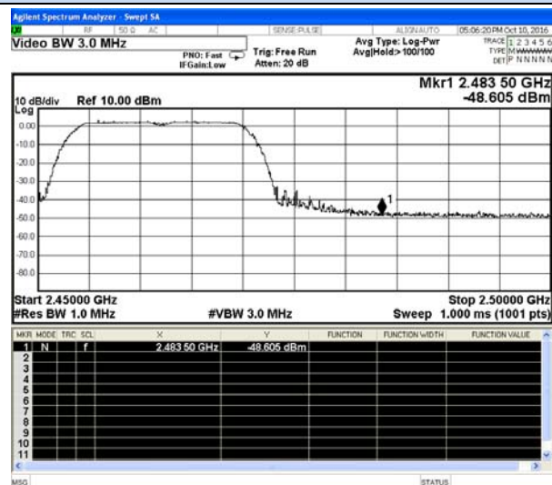
802.11g Chain 0-High channel(Peak)
