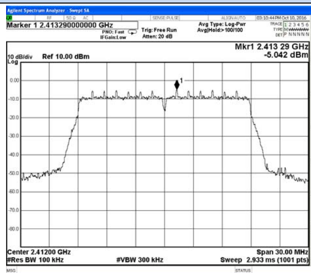
802.11n-HT20 Chain 1-Low channel Reference
