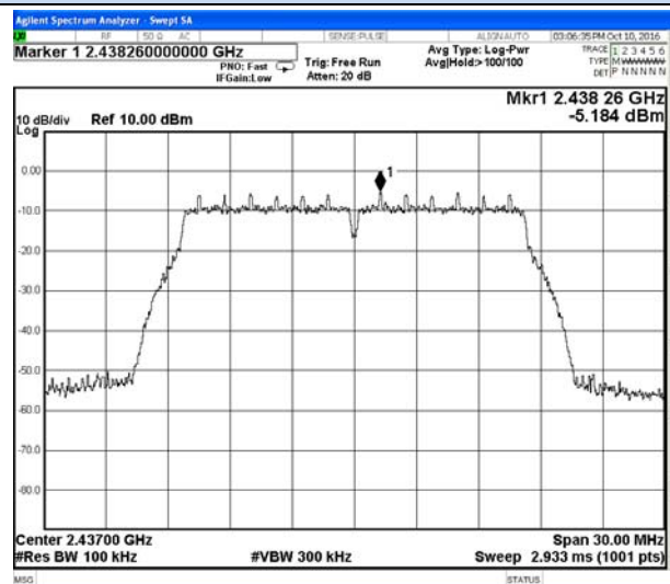
802.11g Chain 1-Middle channel Reference
