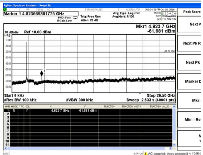
802.11b Chain 0-Low channel
