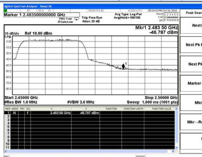
802.11n-HT20 Chain 1-High channel(Peak)
