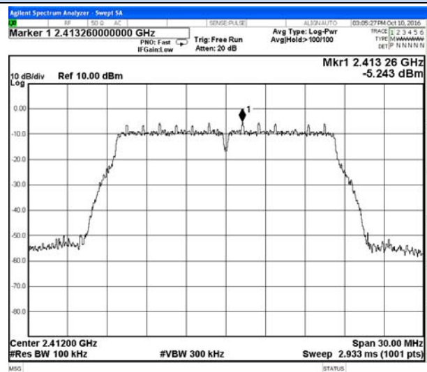
802.11g Chain 0-Low channel Reference
