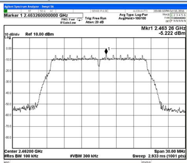
802.11g Chain 0-High channel Reference
