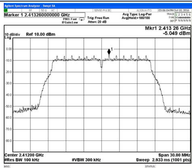
802.11g Chain 1-Low channel Reference
