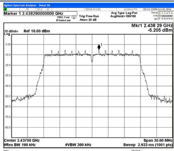
802.11n-HT20 Chain 0-Middle channel Reference
