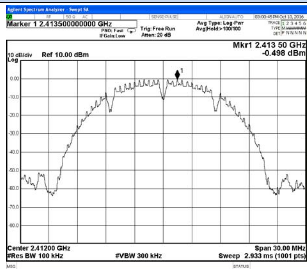
802.11b Chain 1-Low channel Reference
