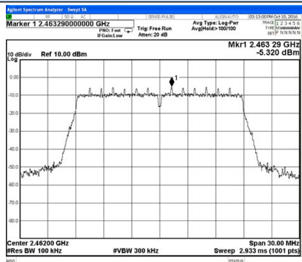
802.11n-HT20 Chain 0-High channel Reference
