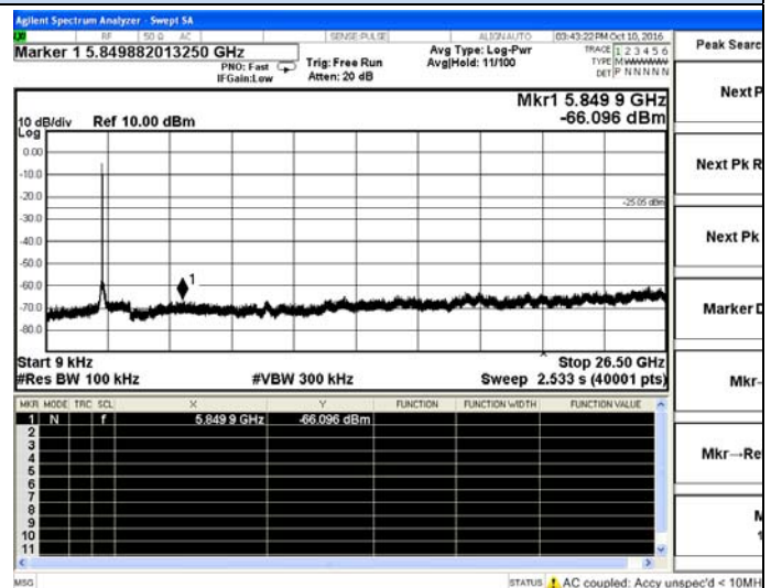
802.11g Chain 1-Low channel
