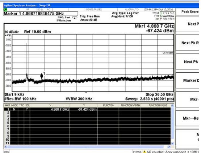
802.11g Chain 1-Middle channel
