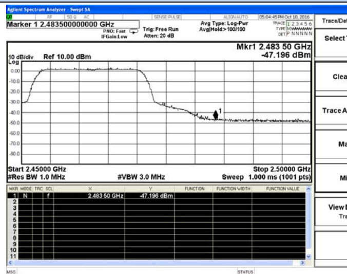
802.11n-HT20 Chain 0-High channel(Peak)
