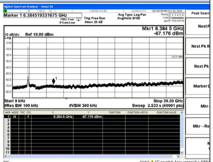
802.11n-HT20 Chain 1-Middle channel
