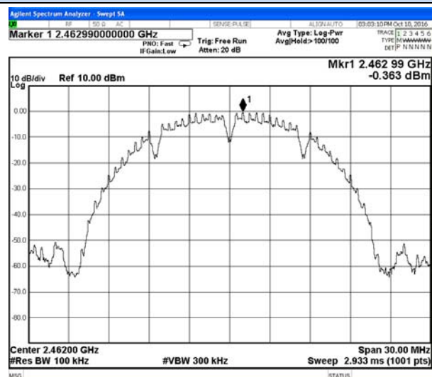
802.11b Chain 1-High channel Reference
