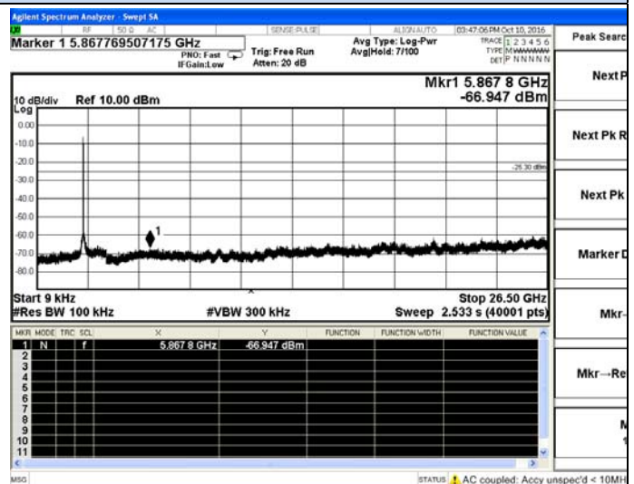
802.11n-HT20 Chain 0-Low channel
