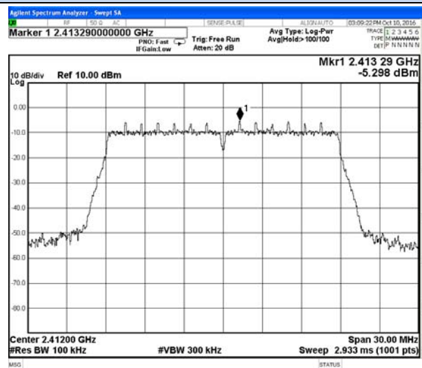
802.11n-HT20 Chain 0-Low channel Reference
