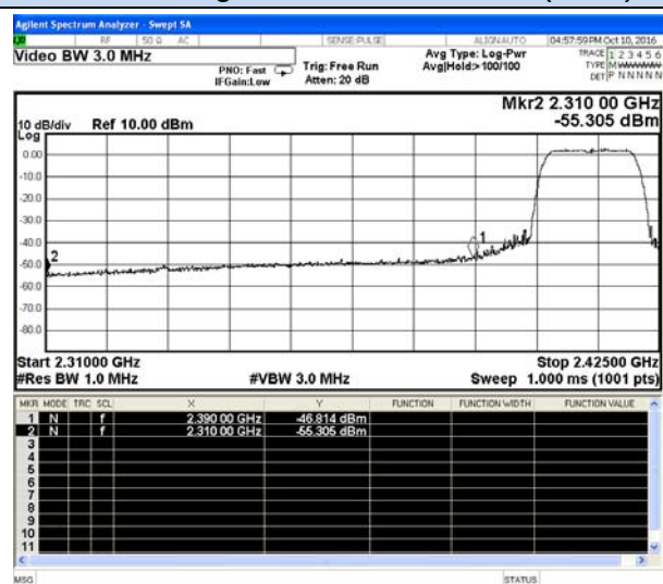
802.11g Chain 1-Low channel(Peak)
