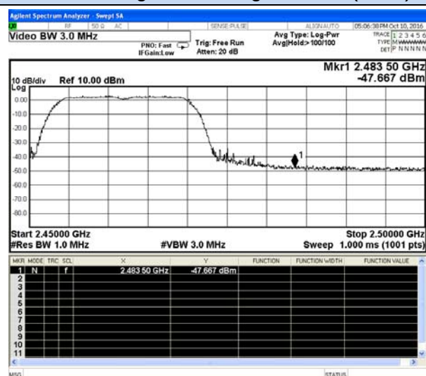
802.11g Chain 1-High channel(Peak)
