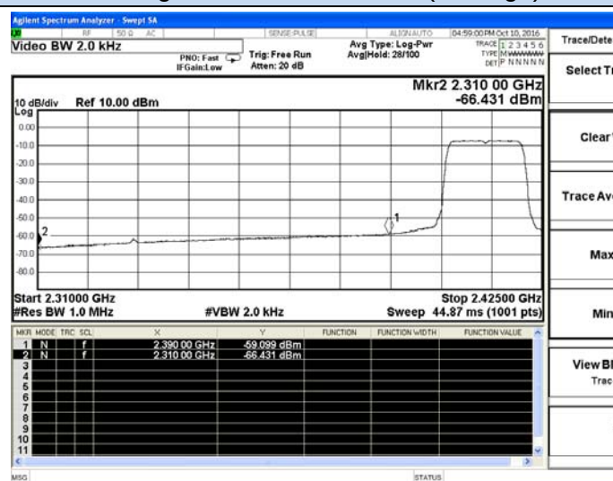
802.11g Chain 1-Low channel(Average)
