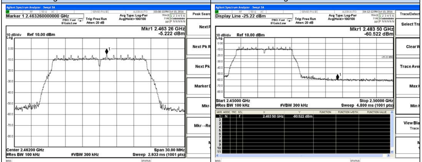
802.11g Chain 0-High channel Reference
