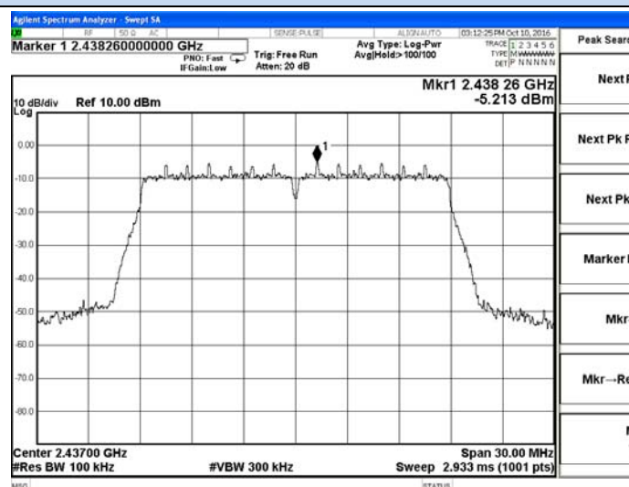
802.11n-HT20 Chain 1-Middle channel Reference
