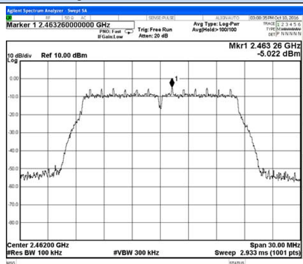
802.11g Chain 1-High channel Reference
