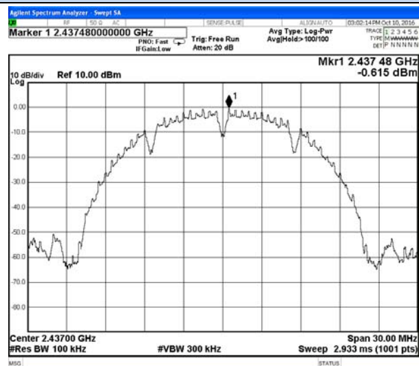
802.11b Chain 1-Middle channel Reference
