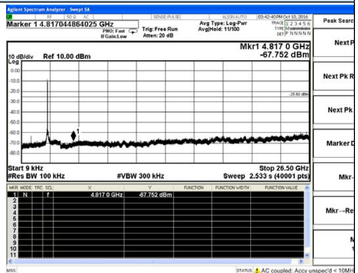
802.11g Chain 0-Low channel
