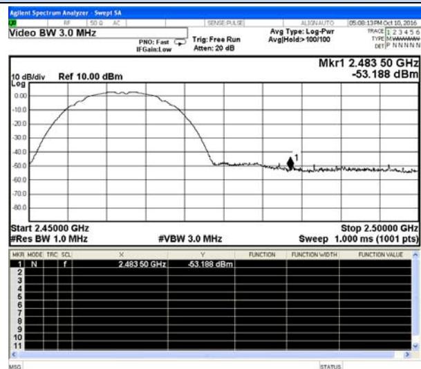
802.11b Chain 1-High channel(Peak)
