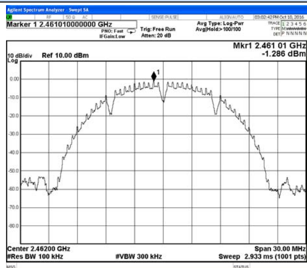
802.11b Chain 0-High channel Reference
