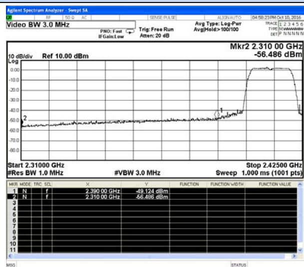
802.11g Chain 0-Low channel(Peak)
