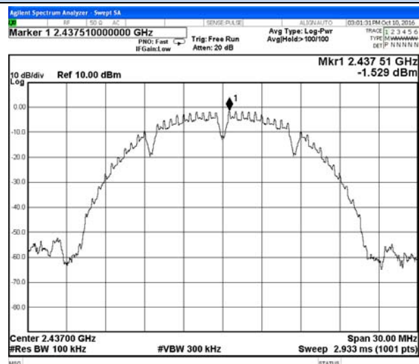
802.11b Chain 0-Middle channel Reference
