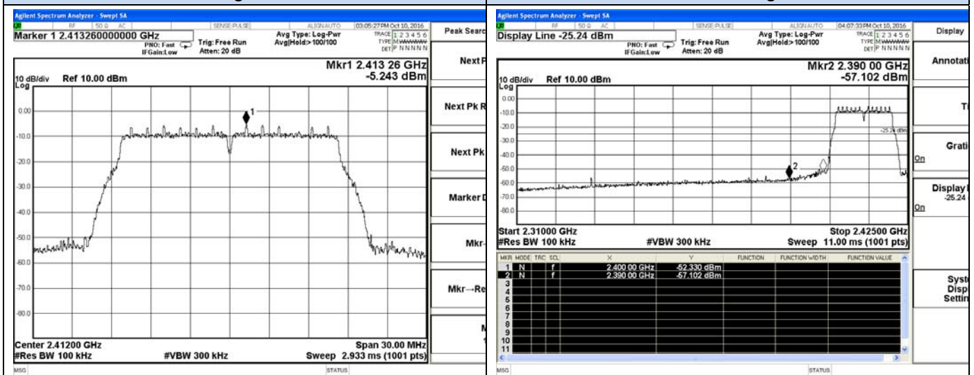
802.11g Chain 0-Low channel Reference
