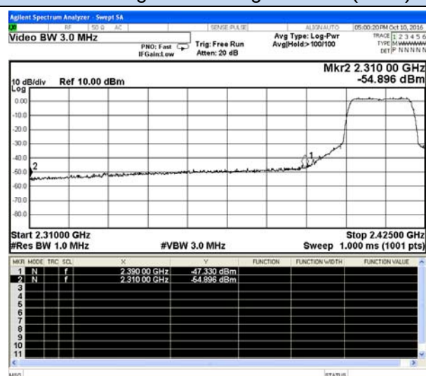
802.11n-HT20 Chain 0-Low channel(Peak)
