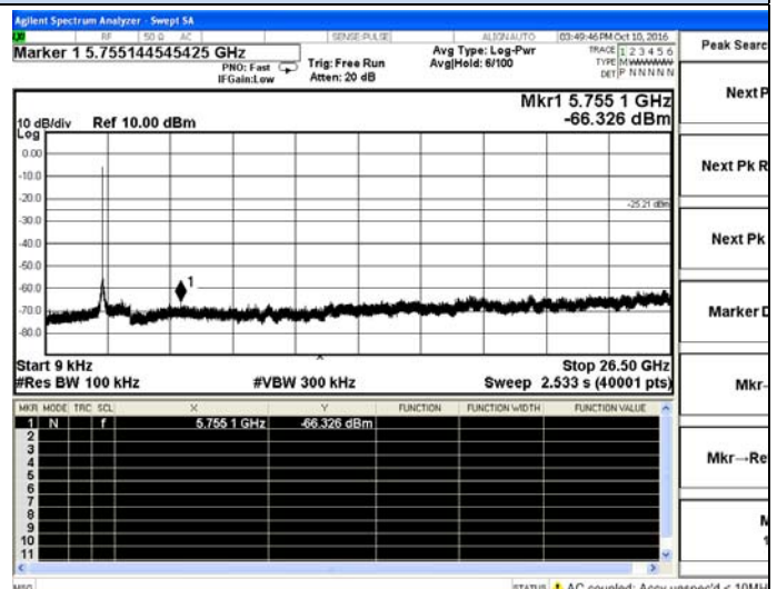
802.11n-HT20 Chain 0-Middle channel
