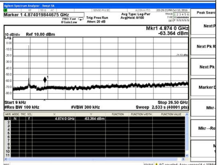
802.11b Chain 0-Middle channel
