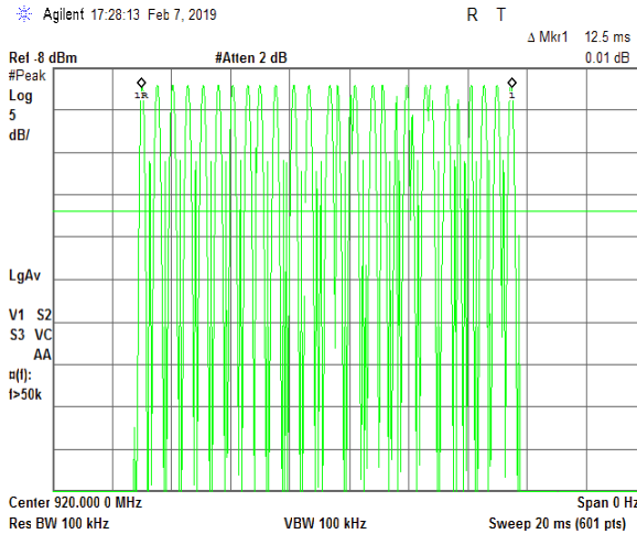
Plot 7.3.13 Transmission burst duration
