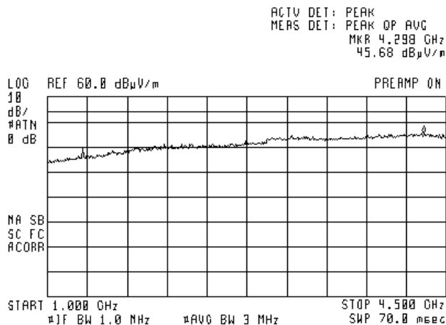
Plot 7.2.8 Radiated emission measurements from 1000 to 4500 MHz
